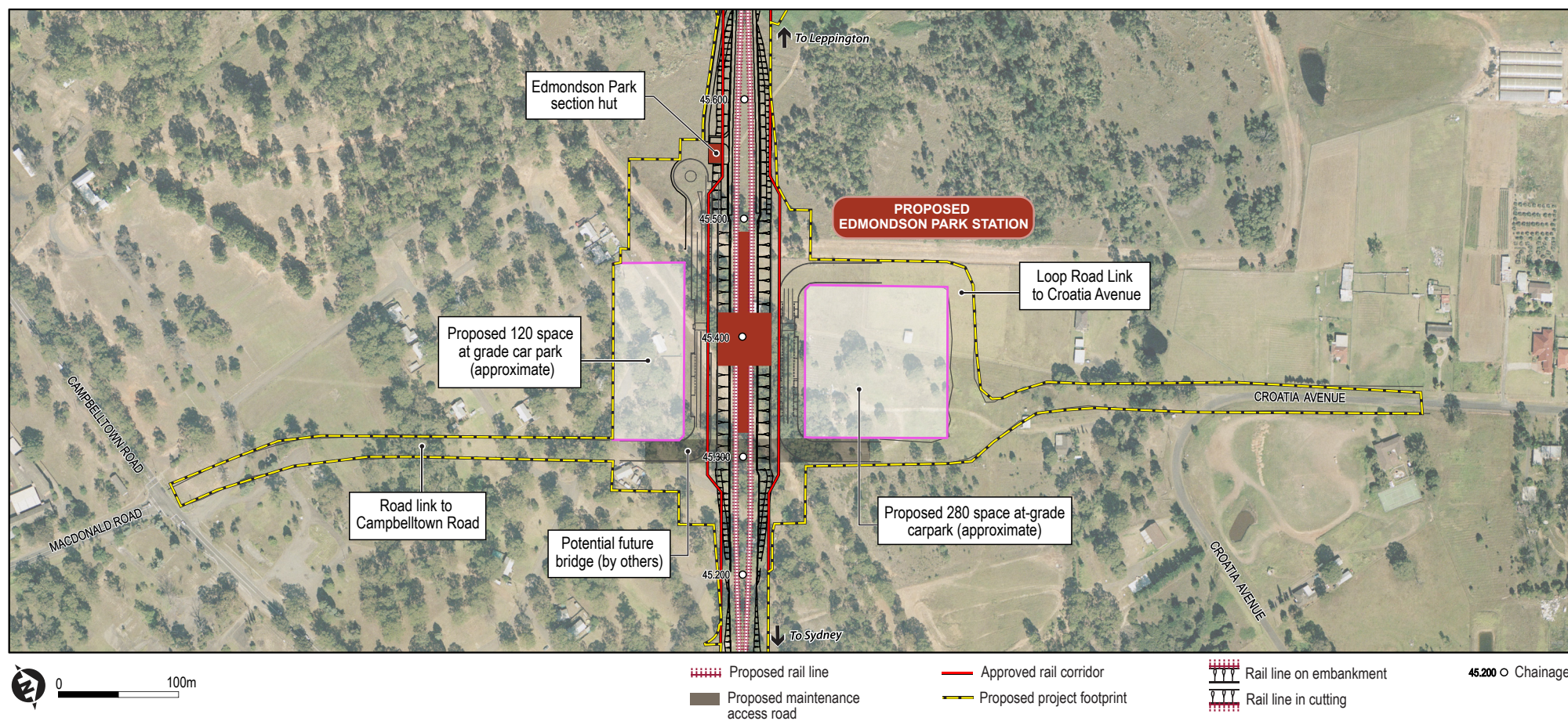
Figure 6-1q Extent of works at Edmondson Park Station *Note: Indicative only, subject to detailed design
