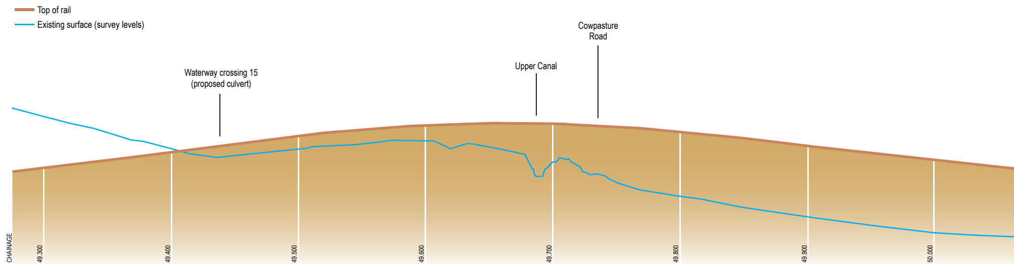
Figure 6-1k The Glenfield to Leppington Rail Line Project *Note: Indicative only, subject to detailed design
