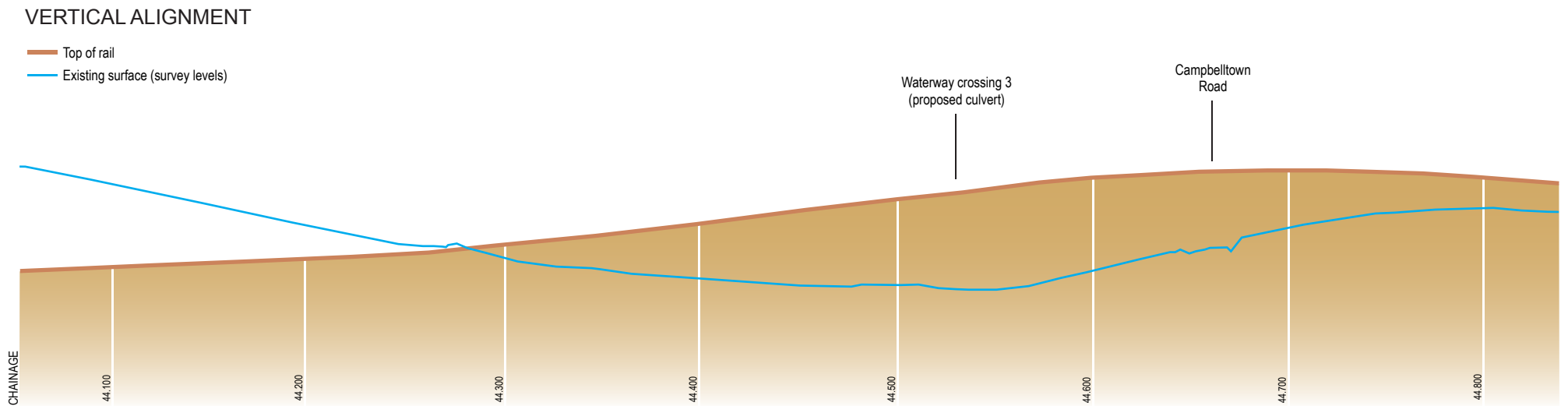
Figure 6-1d The Glenfield to Leppington Rail Line Project *Note: Indicative only, subject to detailed design
