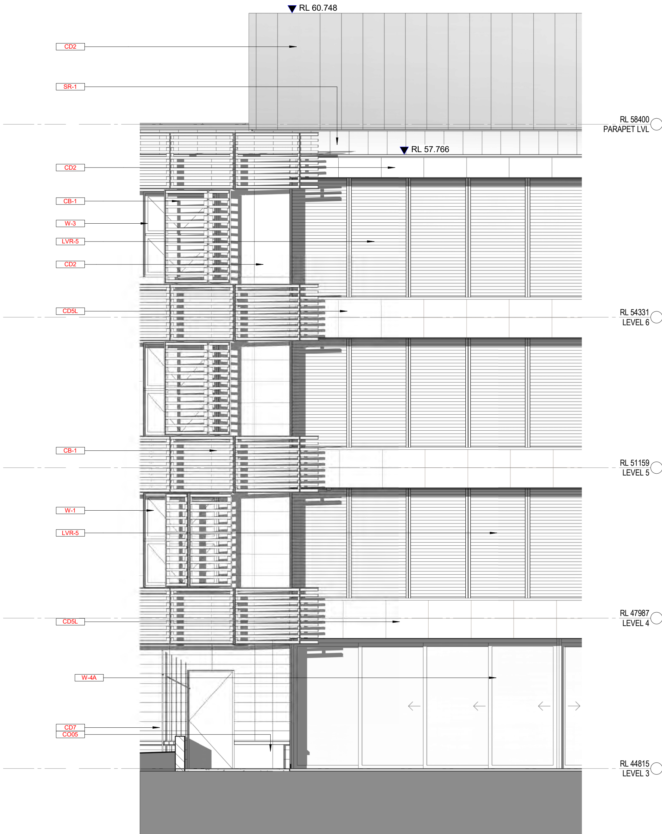
2 BLOCK D EAST FACADE 1 : 50
