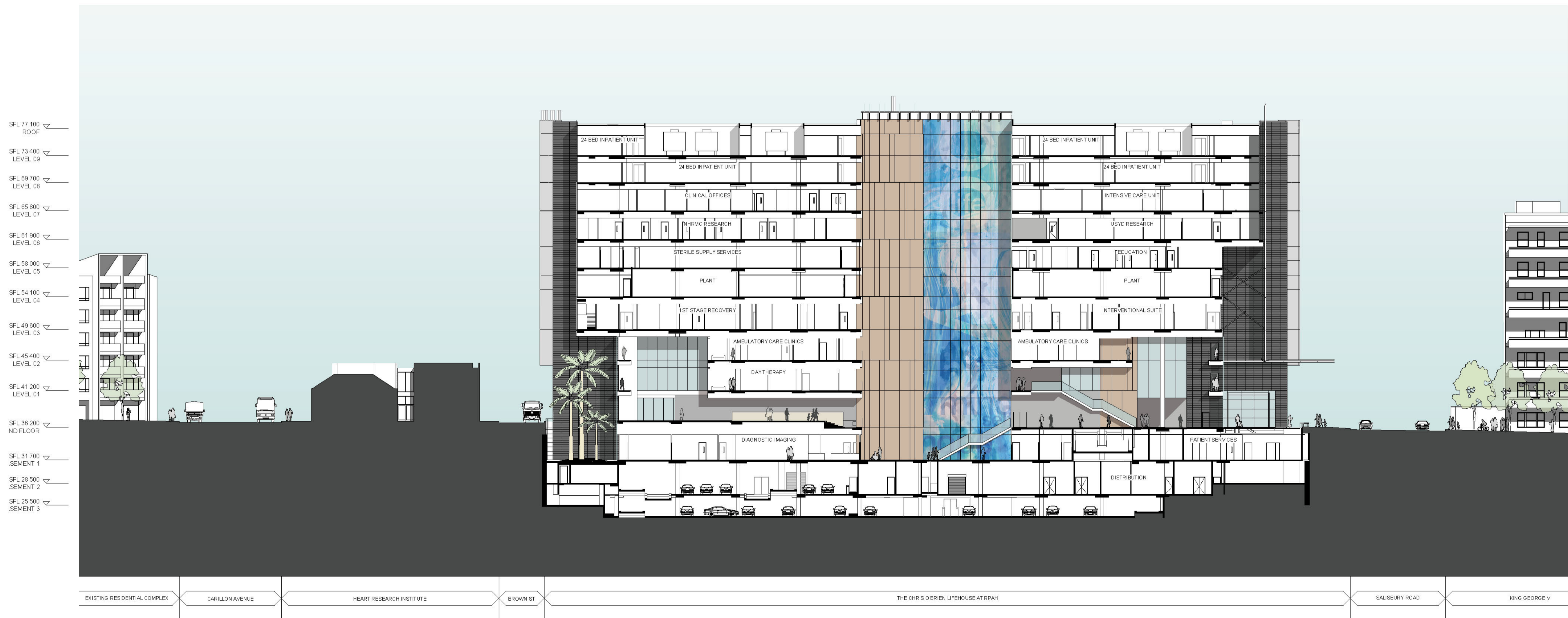
SECTION 1-1
