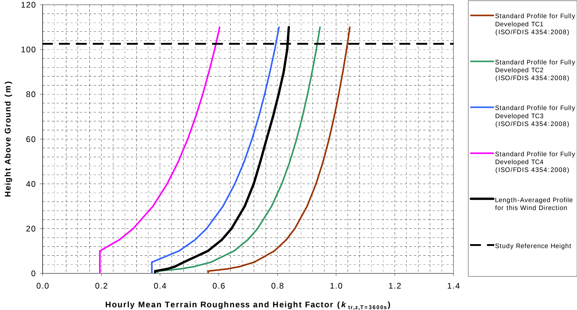
Hourly Mean Velocity Profile for North-Easterly Winds
