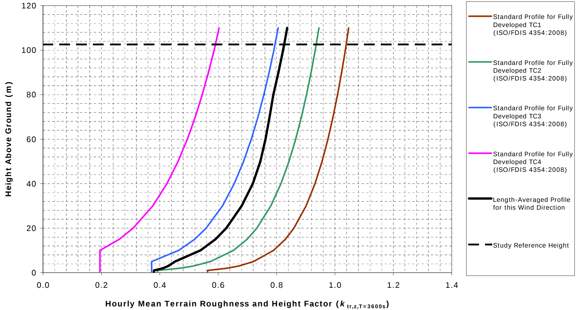
Hourly Mean Velocity Profile for North-Westerly Winds
