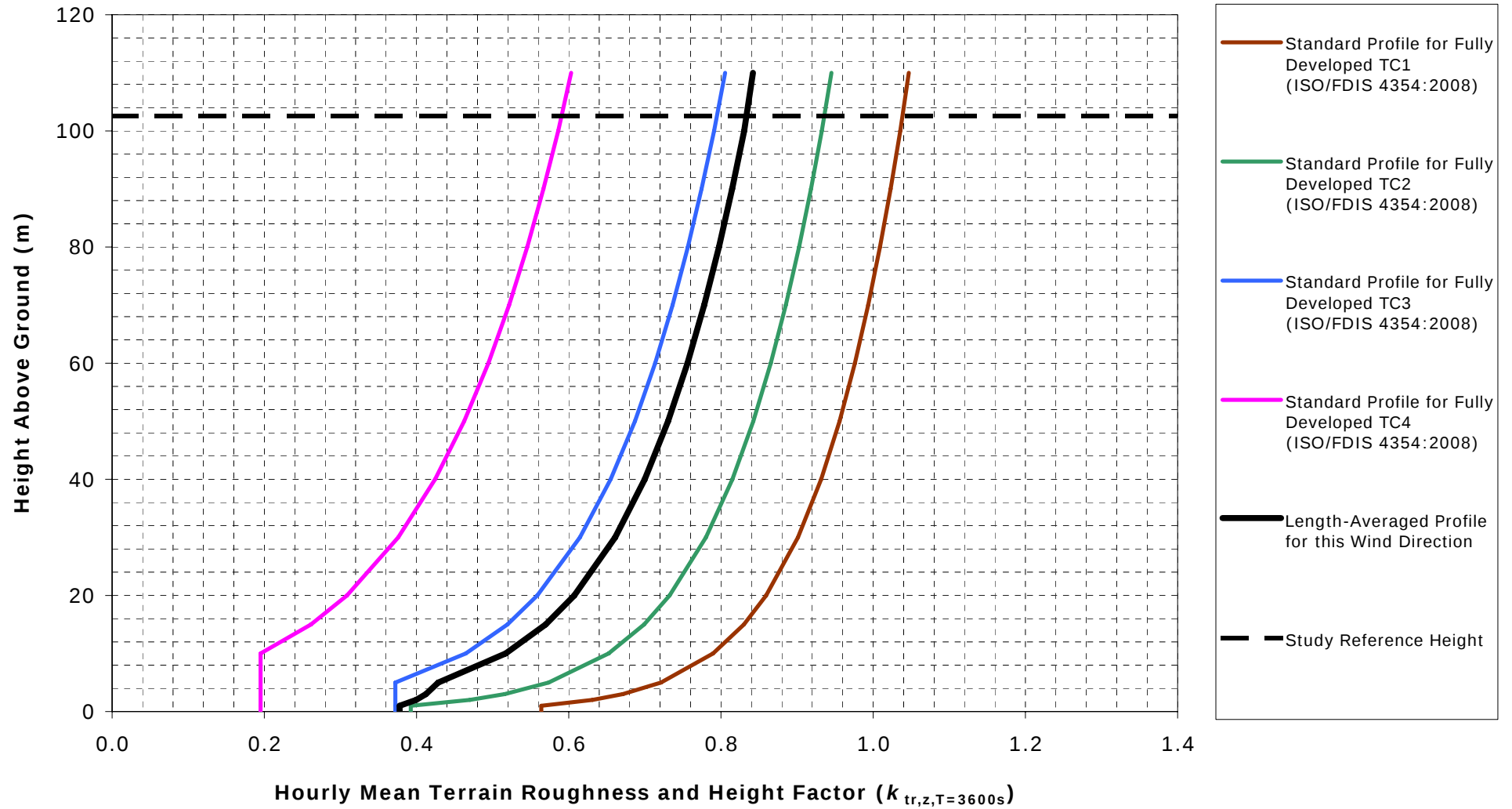
Hourly Mean Velocity Profile for South-Westerly Winds
