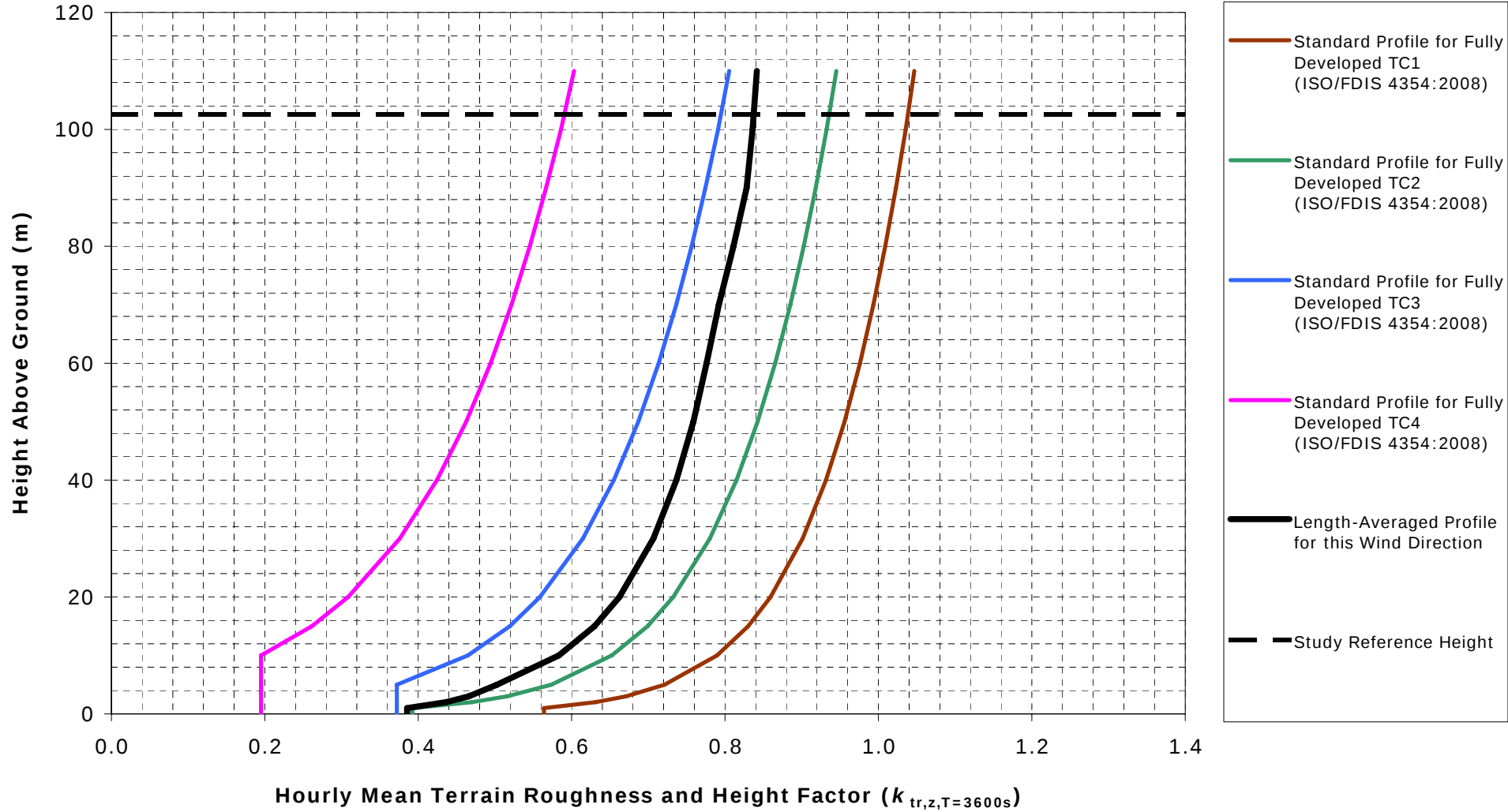
Hourly Mean Velocity Profile for Northerly Winds
