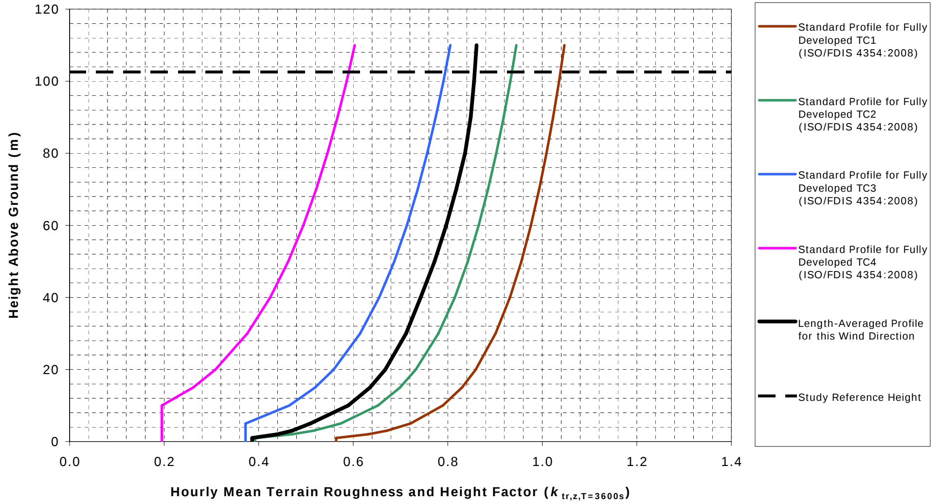
Hourly Mean Velocity Profile for East-North-Easterly Winds
