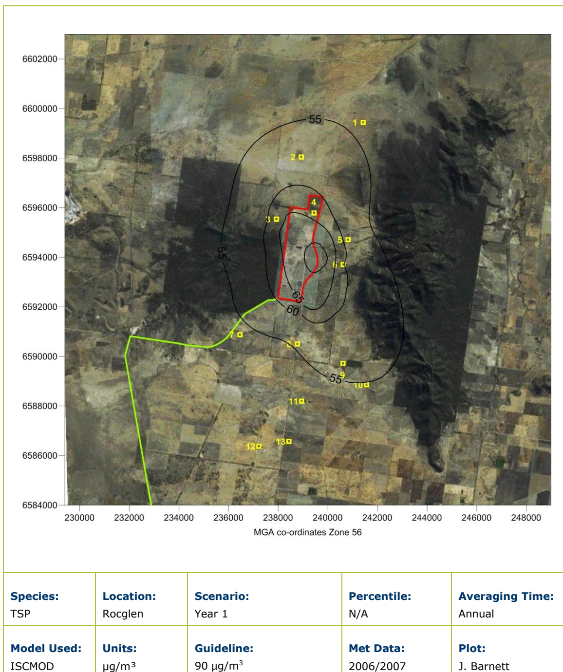
Figure 7.2: Predicted annual average TSP concentrations due to emissions from the Rocglen Mine and other sources – Year 1
