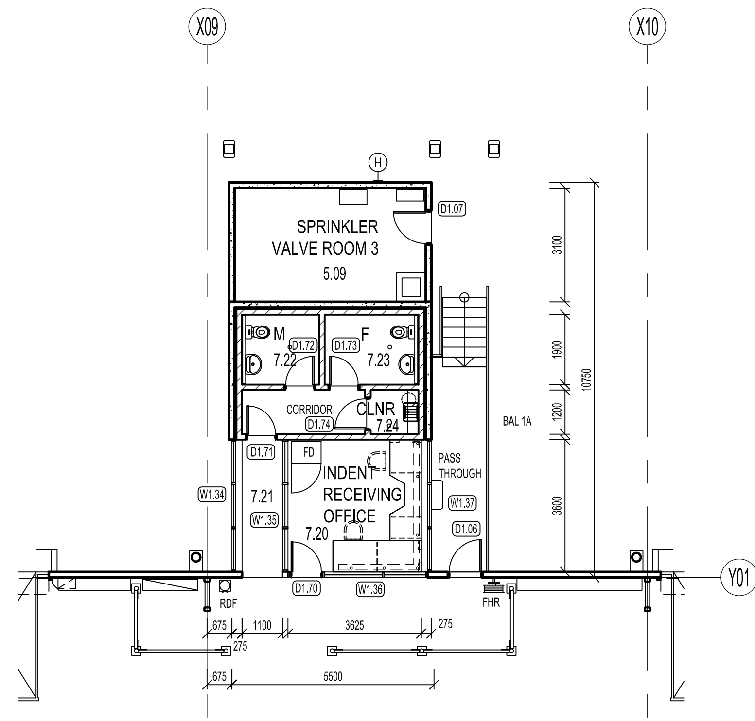
01 FLOOR PLAN INDENT RECEIVING OFFICE
