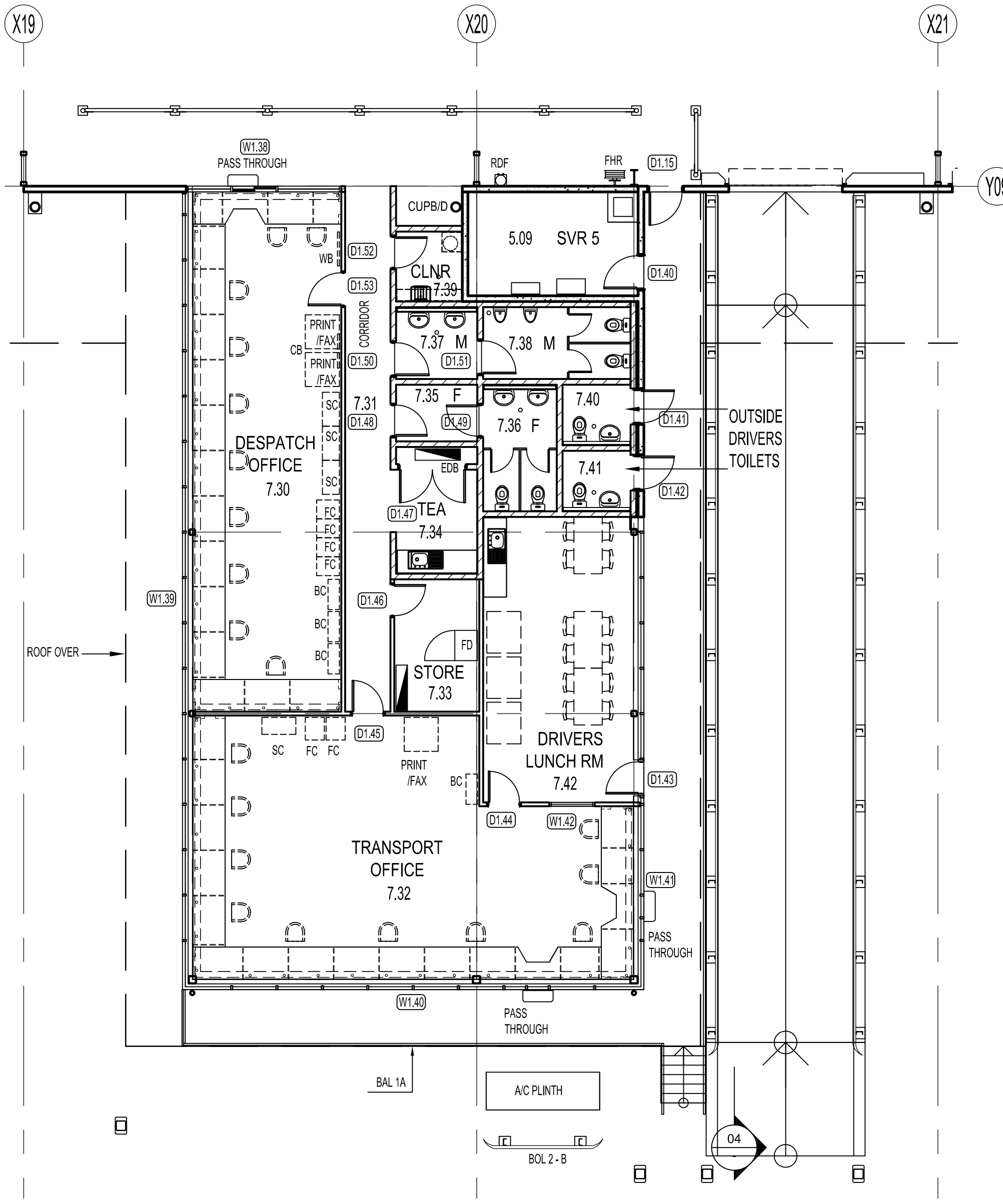
04 FLOOR PLAN DESPATCH OFFICE
