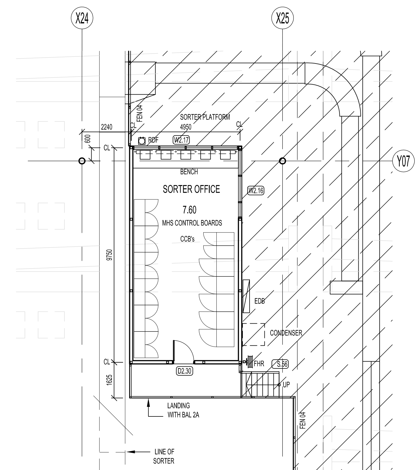
06 FLOOR PLAN SORTER OFFICE (ON SORTER PLATFORM)
