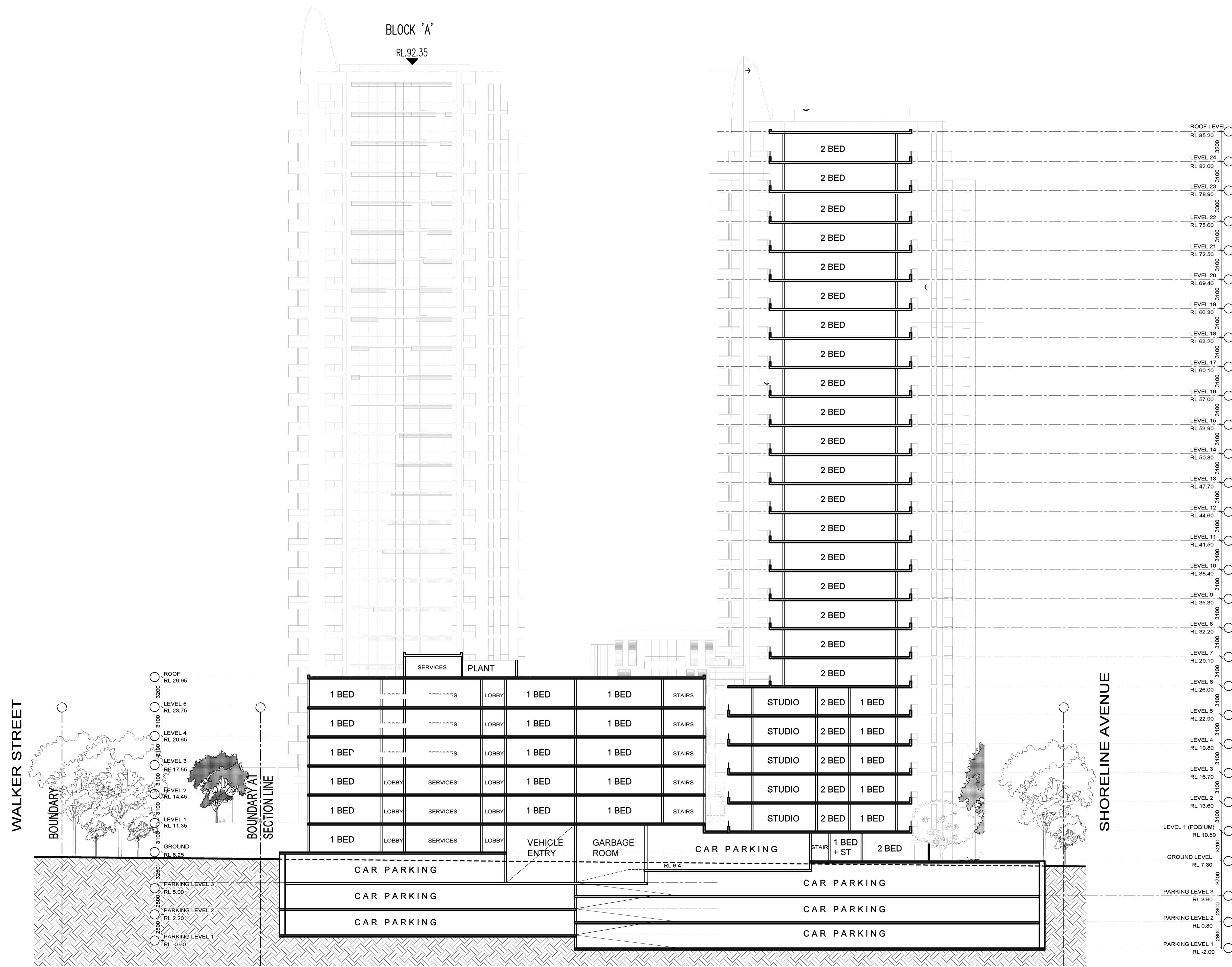
SITE SECTION C-C SCALE 1:200
