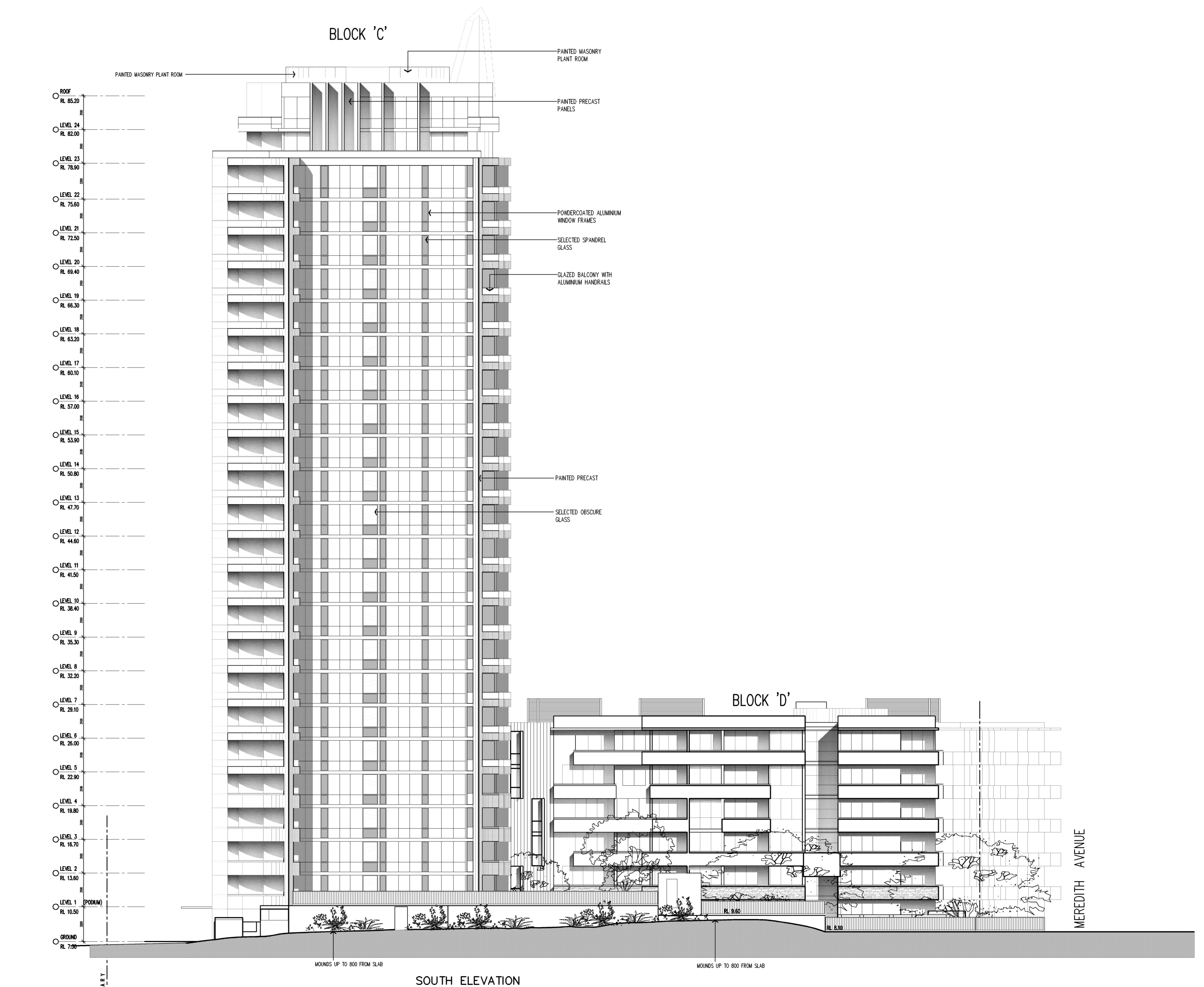
BUILDING C ELEVATIONS SHEET 2 SCALE 1:200
