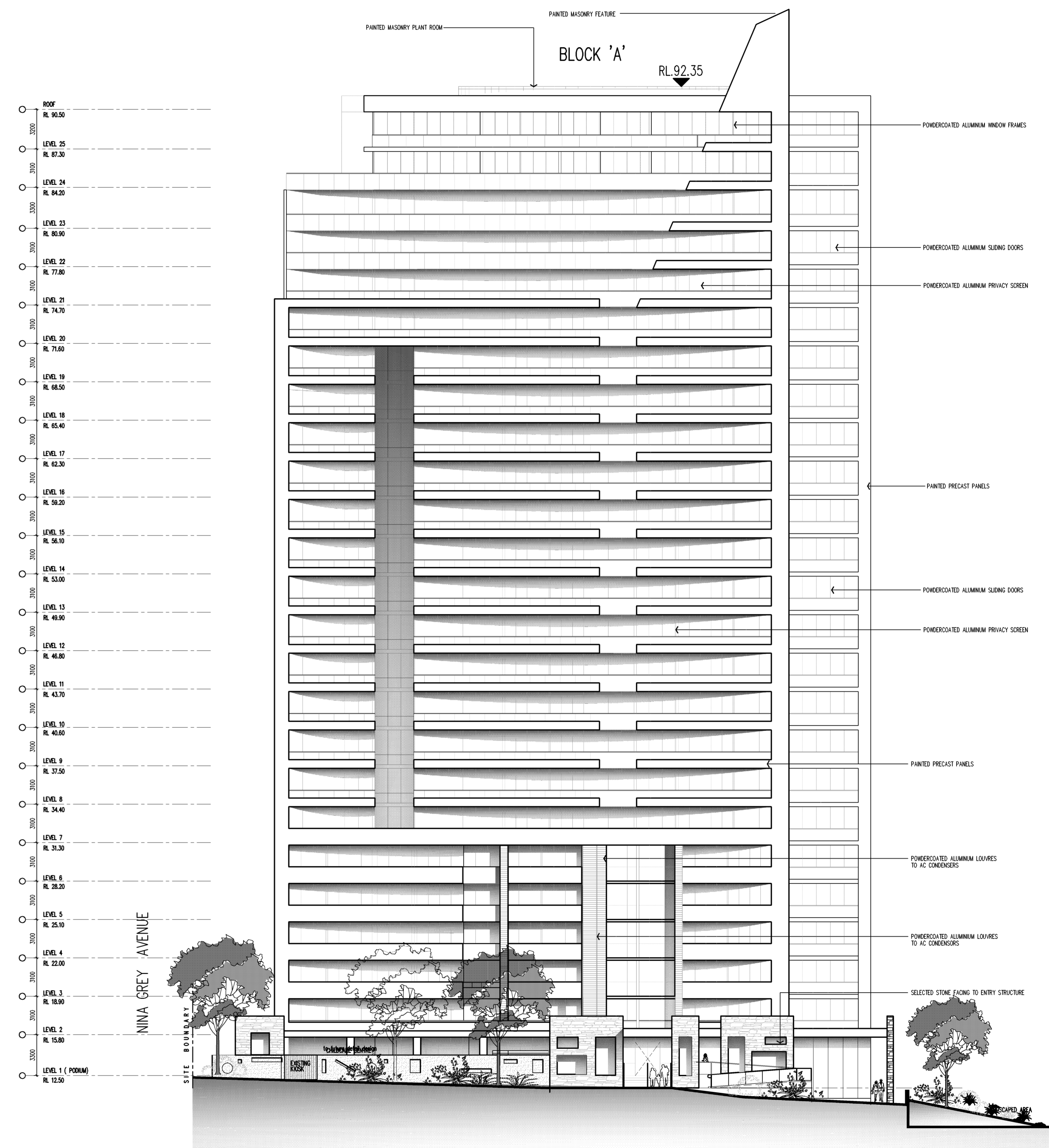
EAST ELEVATION
