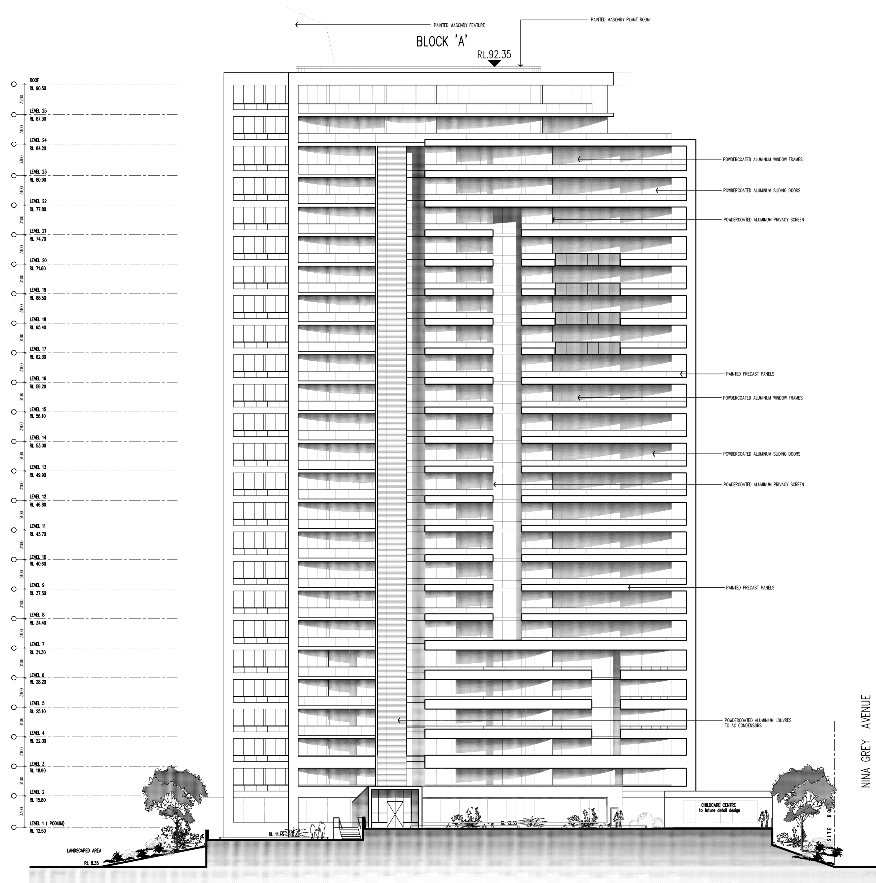
WEST ELEVATION
