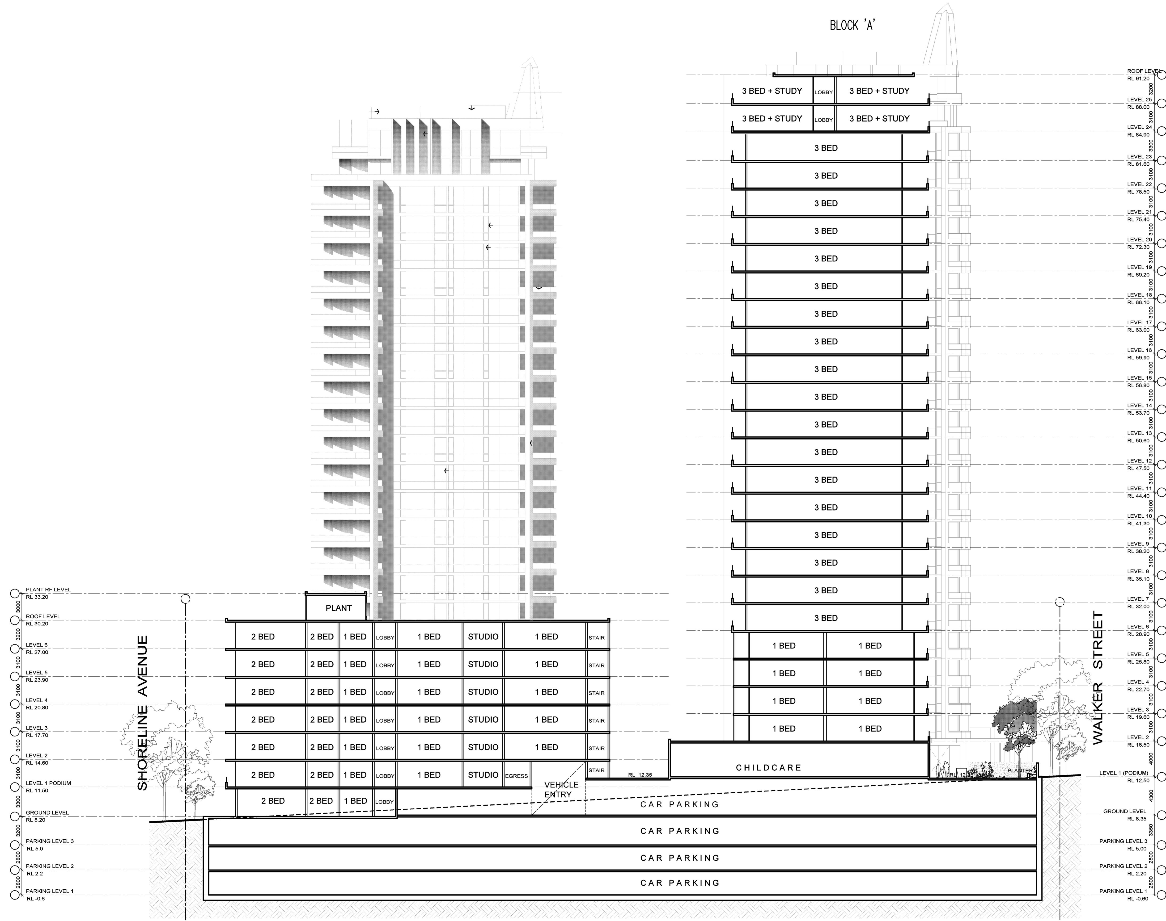
SITE SECTION B-B SCALE 1:200
