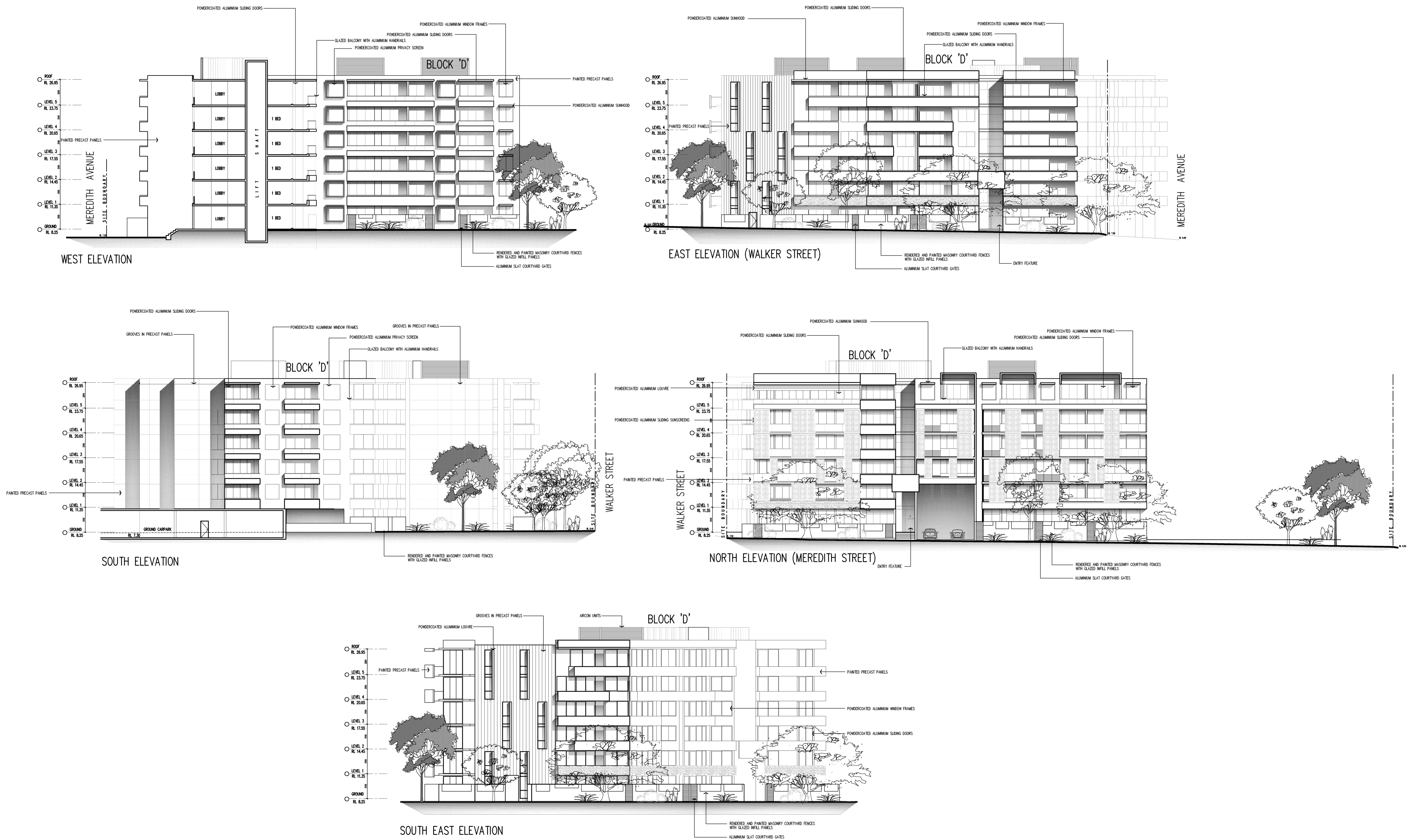
BUILDING D ELEVATIONS SCALE 1:200
