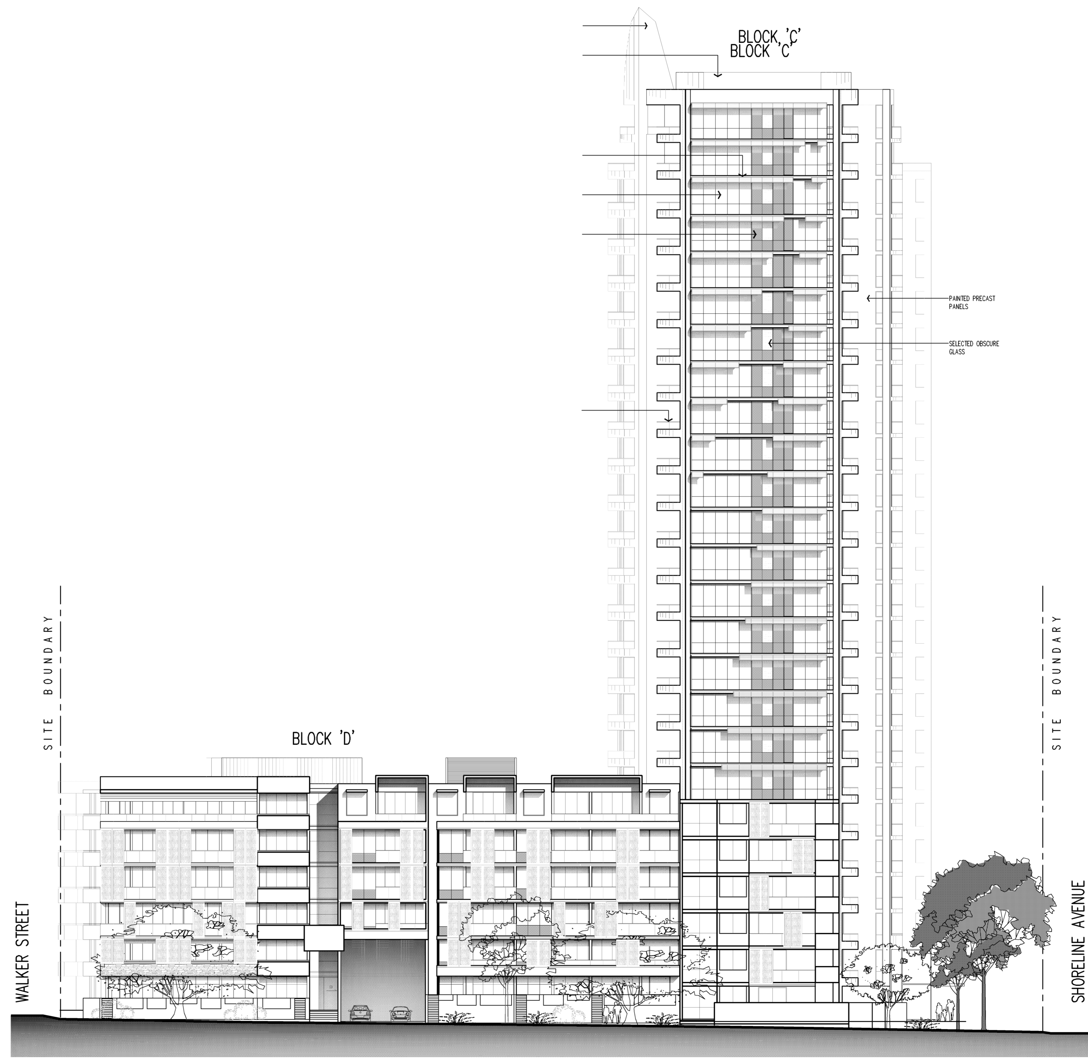
MEREDITH AVE ELEVATION SCALE 1:200
