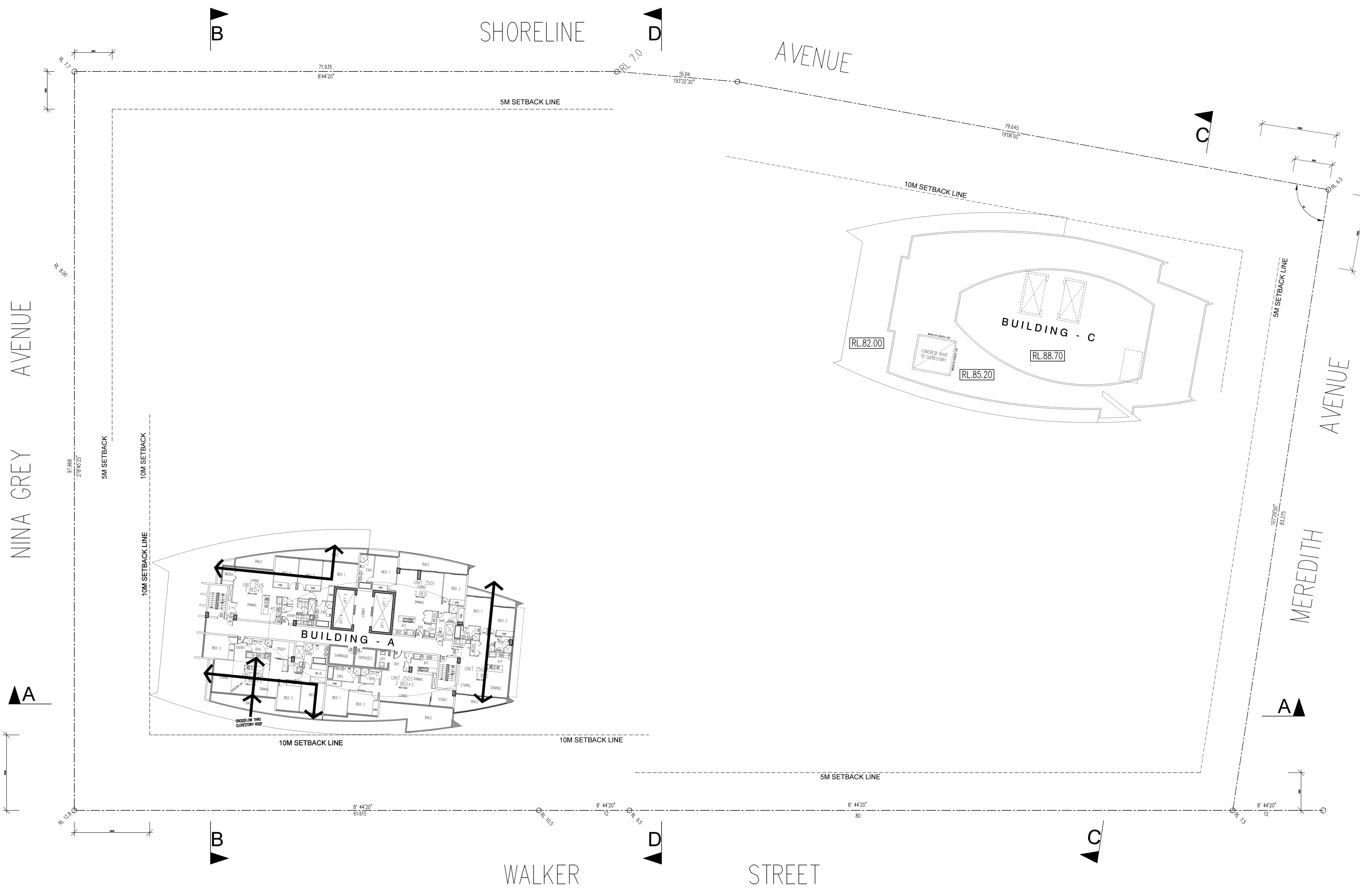
CROSS VENTILATION LEVEL 25 PLAN SCALE 1:200
