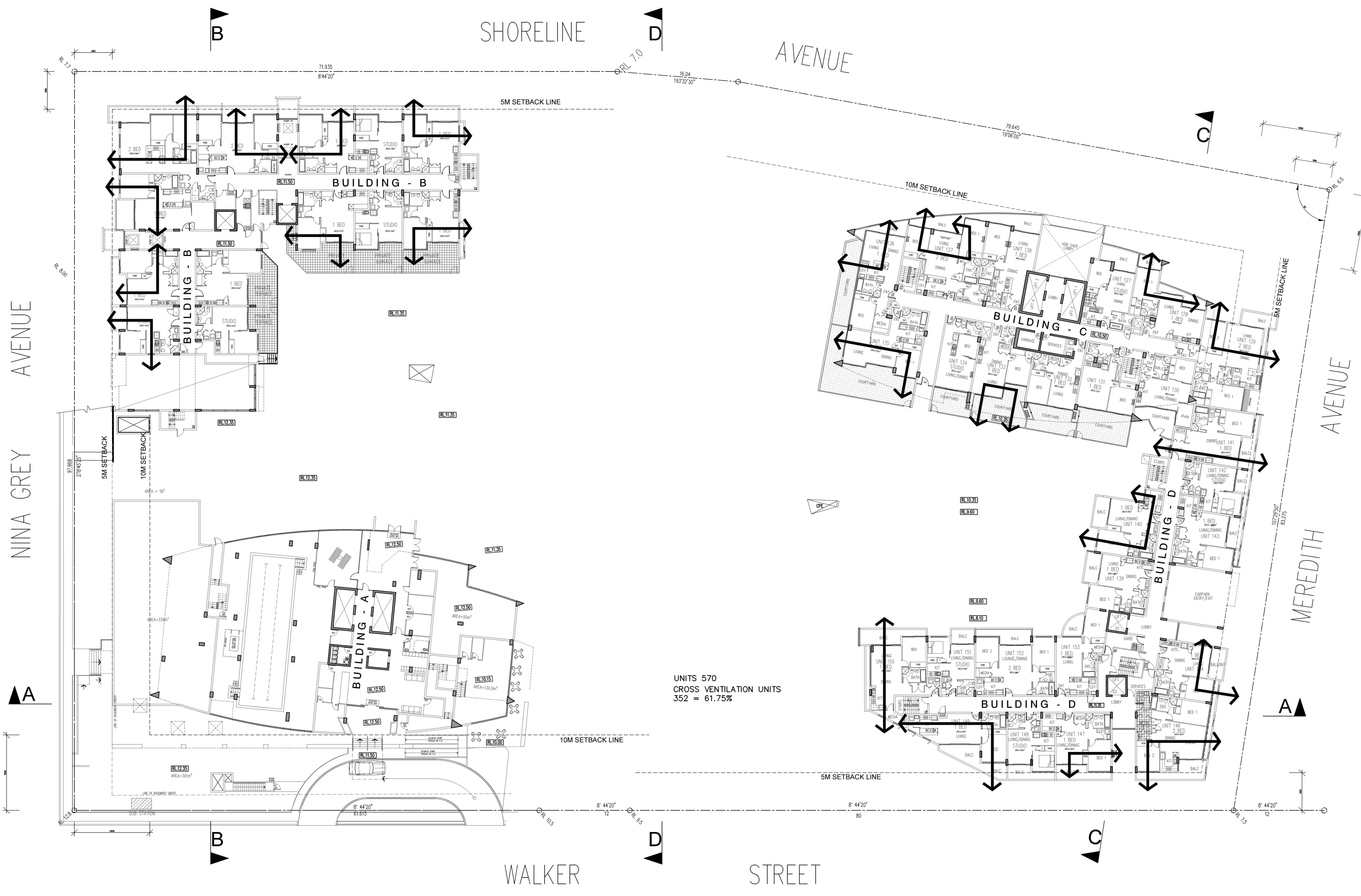
CROSS VENTILATION LEVEL 1 PLAN SCALE 1:200
