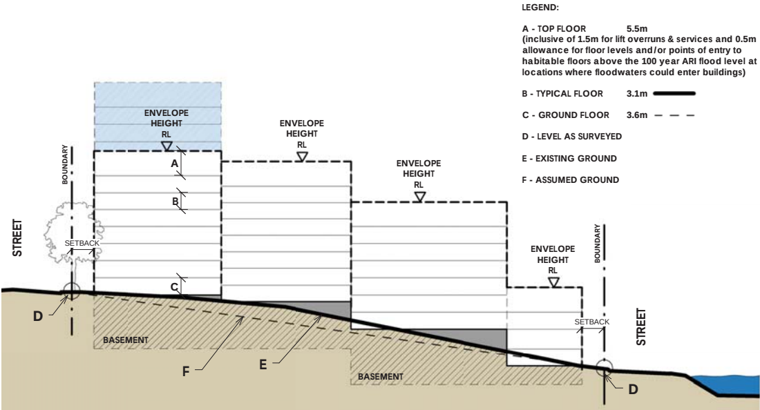
FIGURE 11. CONCEPT PLAN METHOD OF DEFINING HEIGHT
