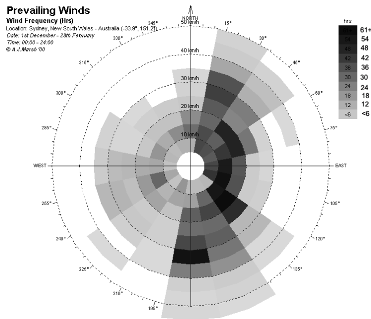
Figure 2: Summer wind velocities and frequencies, Sydney.
