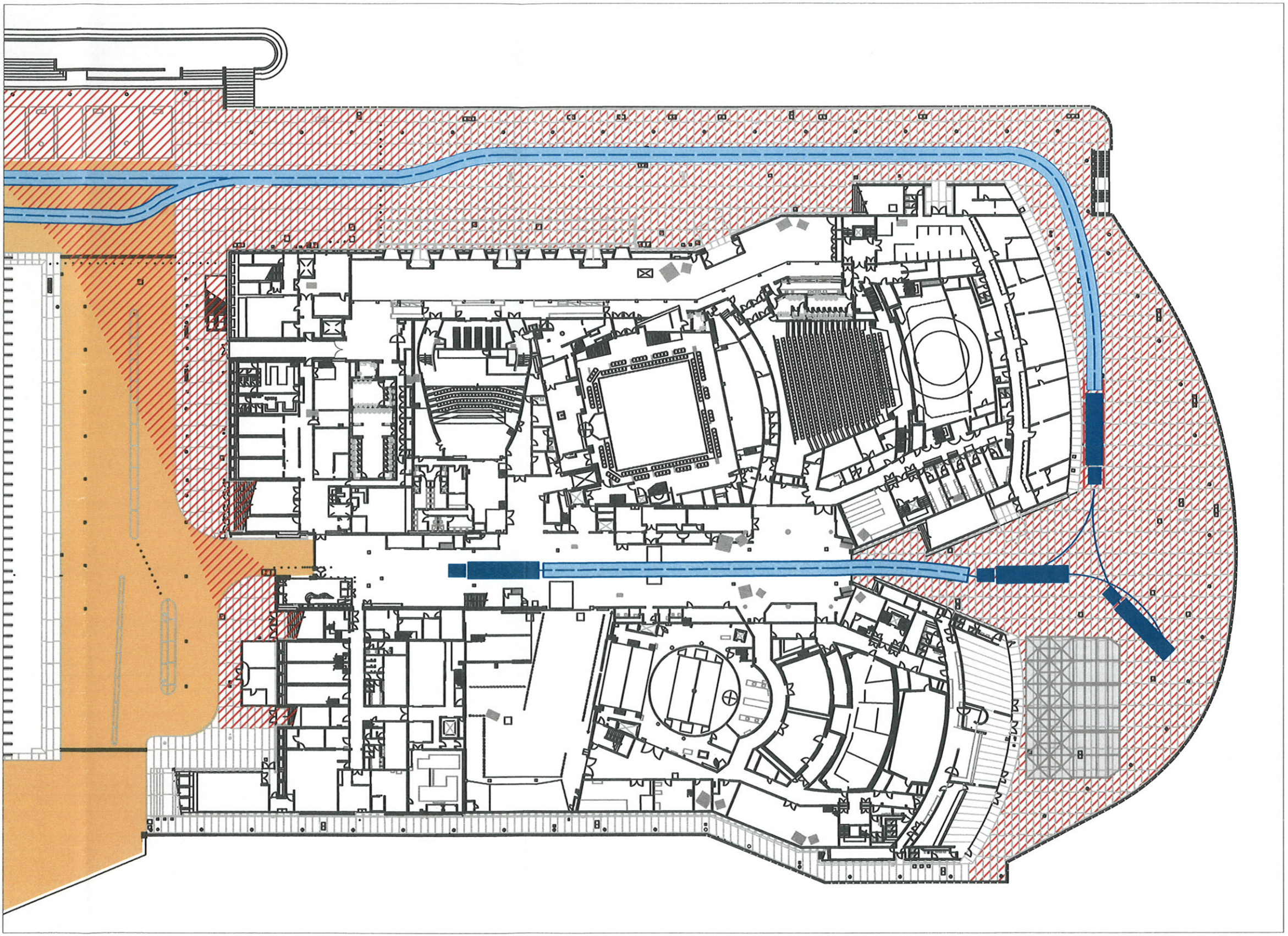
Showing typical truck path via Western & Northern Broadwalks to gain entry to/from Central Passage Red hatch shows shared truck and public pedestrian movement
