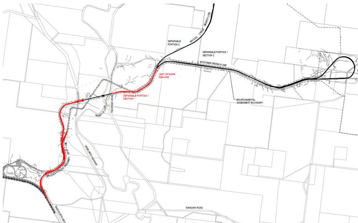
Figure 3: Boggabri Rail Spur Line – incorporating Boggabri Branch Line and Shared Spur Line (Red) and Rail Bridge over Namoi River
