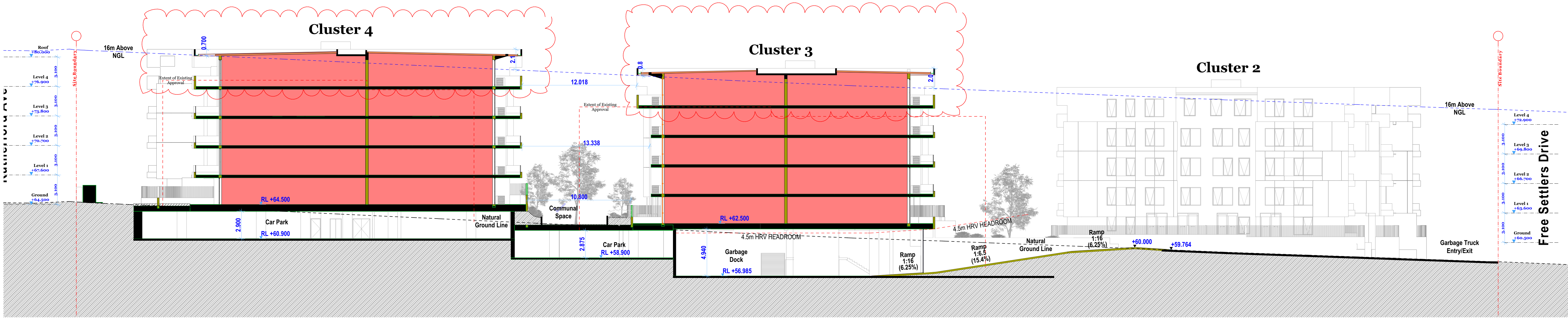
1 Section A 1:200
