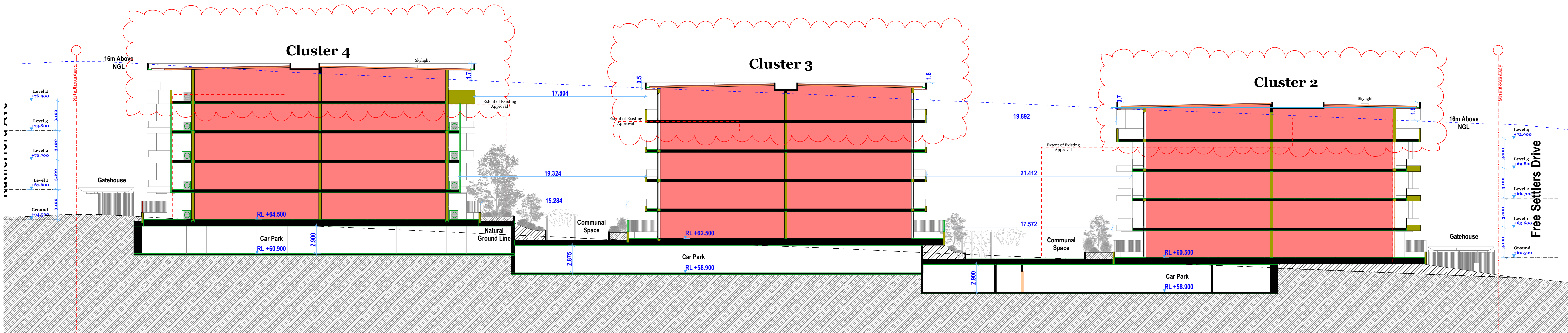
2 Section B 1:200
