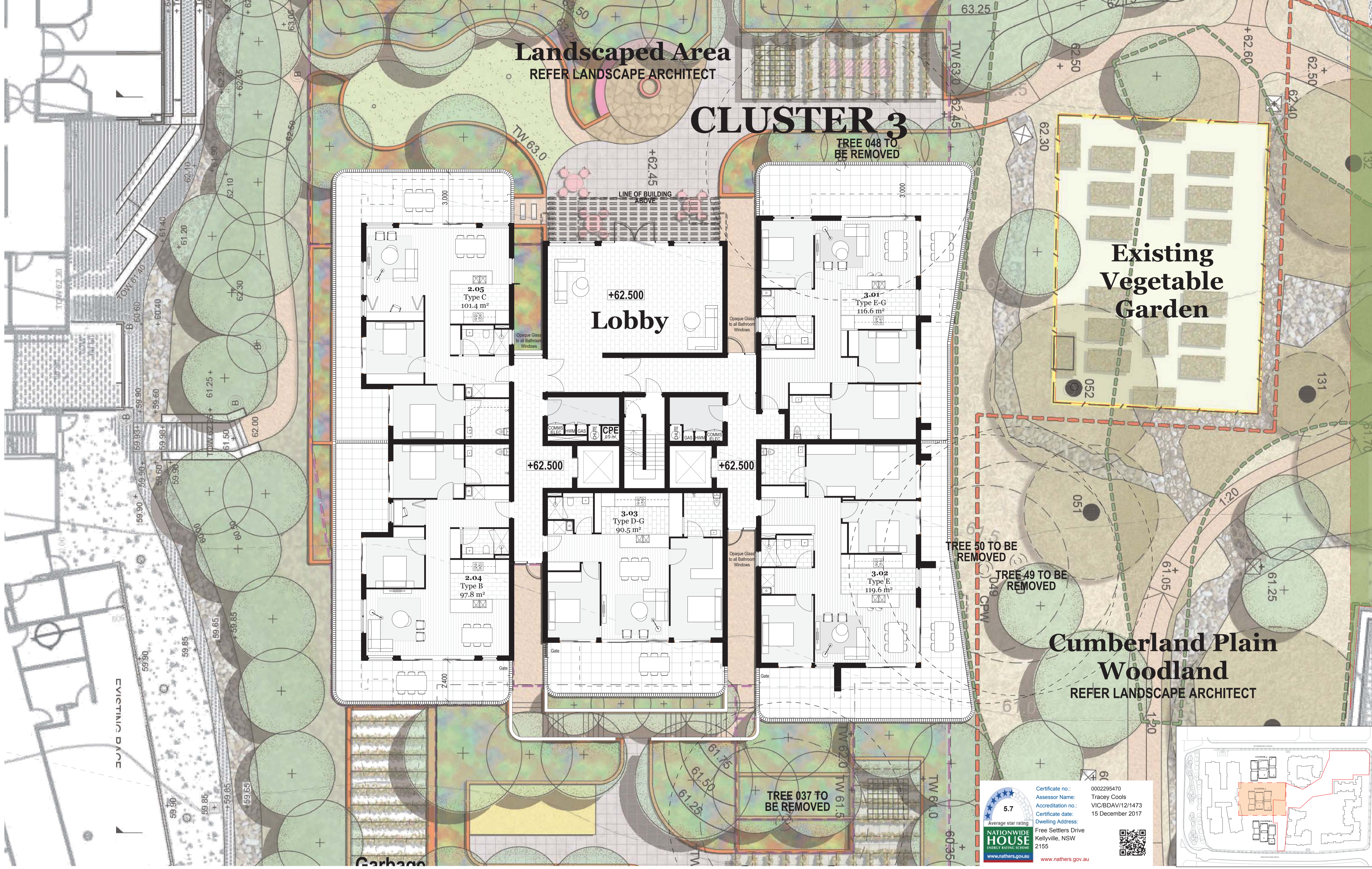
Cluster 3 Ground 1:100
