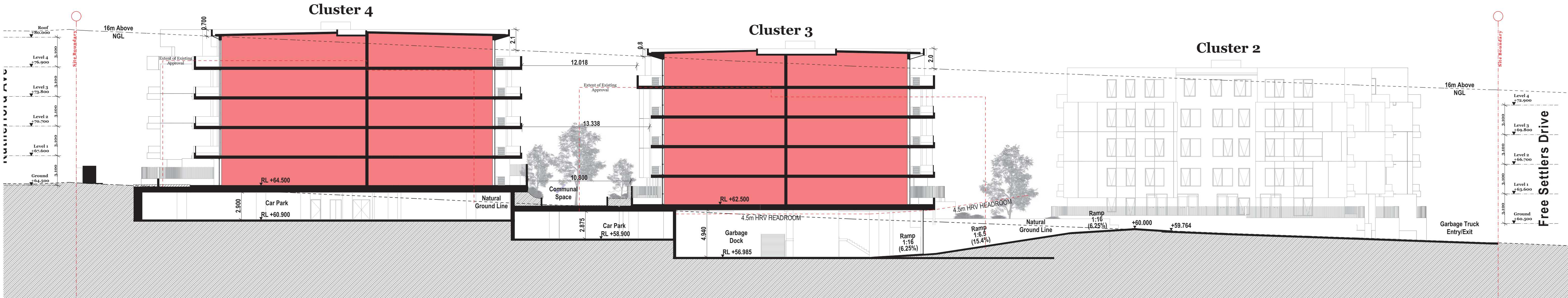
1 Section A 1:200
