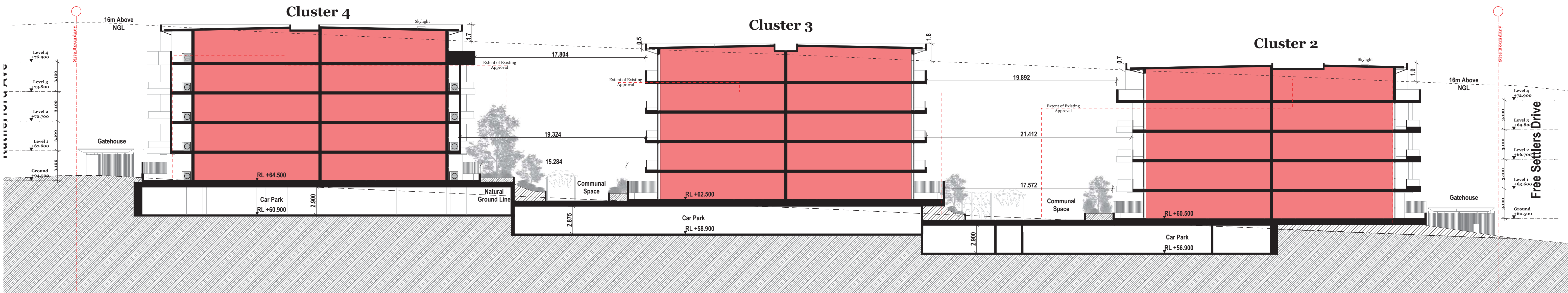
2 Section B 1:200
