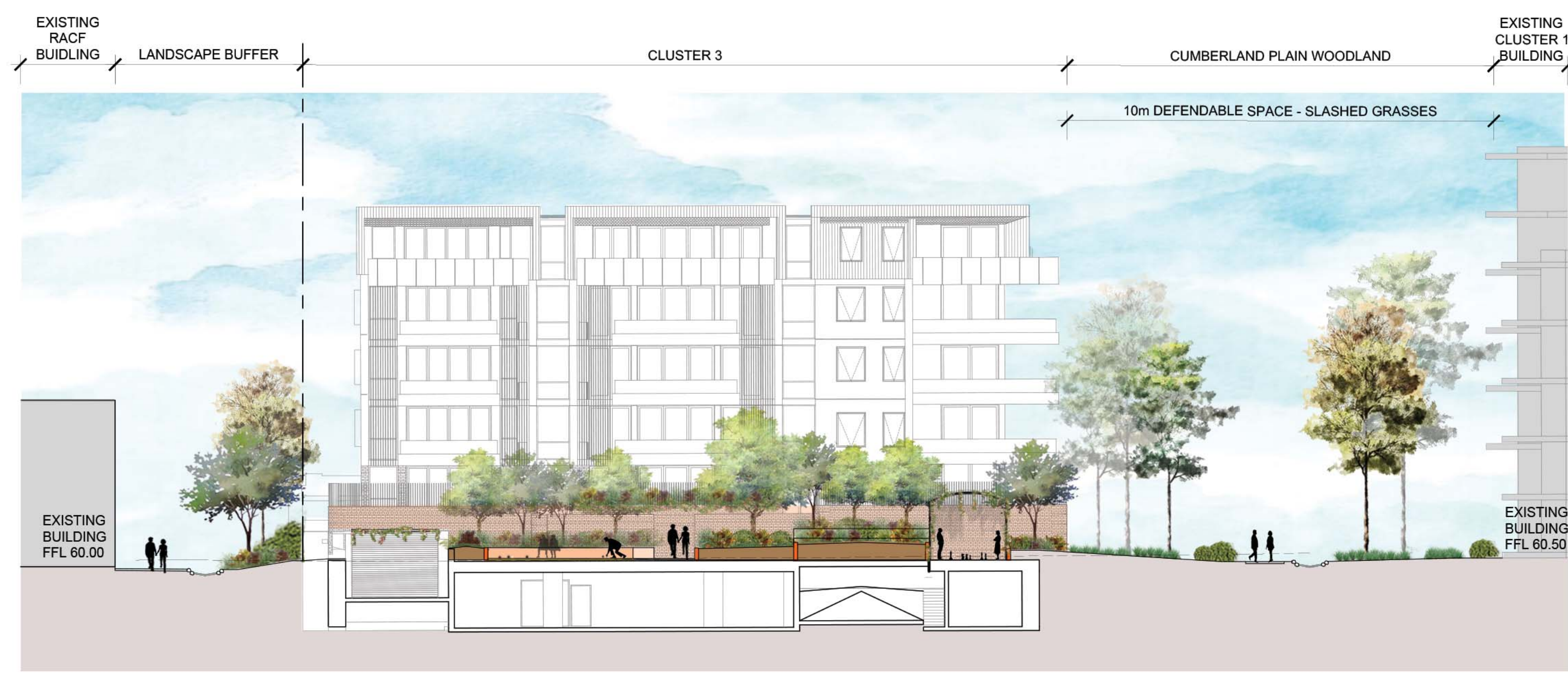
SECTION ELEVATION CC 1:200
