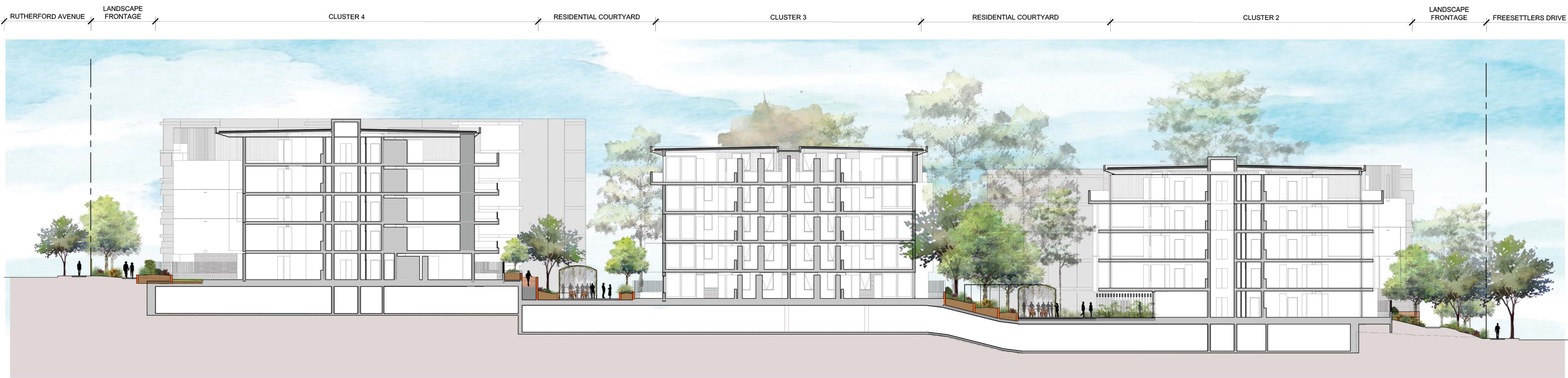
SECTION ELEVATION AA 1:200
