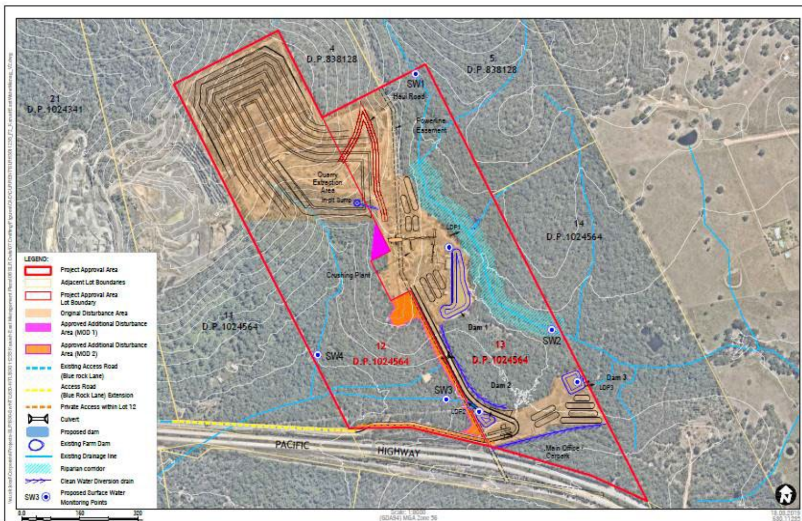
Figure 3 Current Water Management System (Prepared by SLR)
