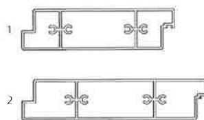
1. Hi-Span 135 blade profile 2. Hi-Span 165 blade profile
