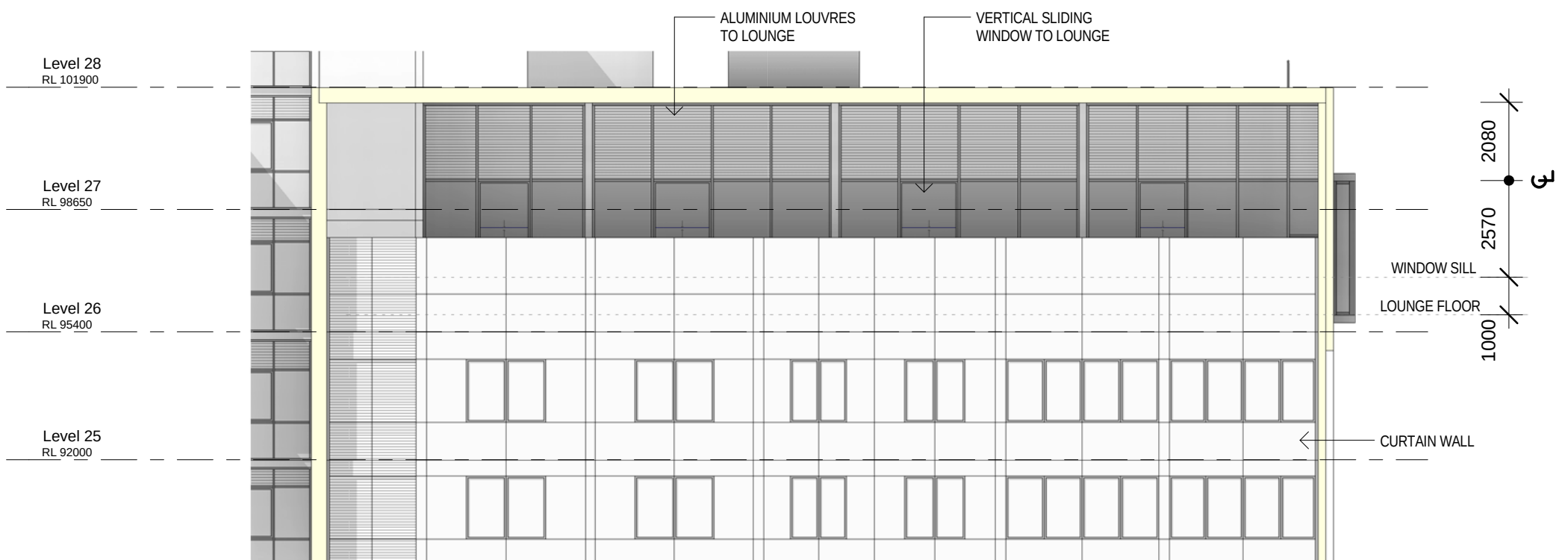
2 WEST ELEVATION OF LOUNGE
