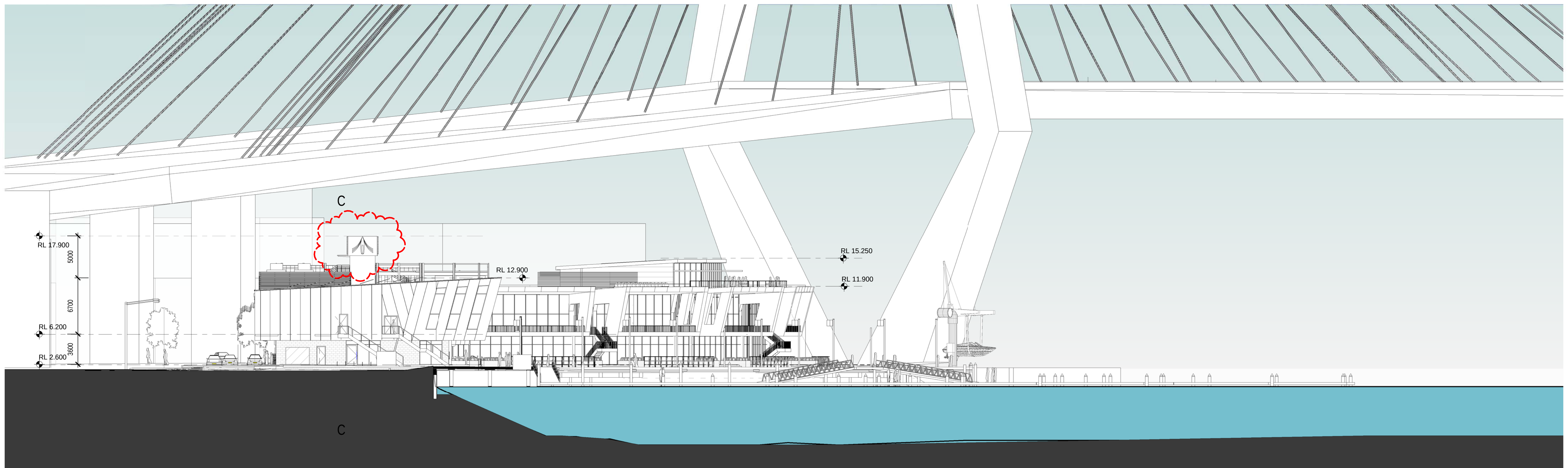
2 WEST ELEVATION 1 : 250
