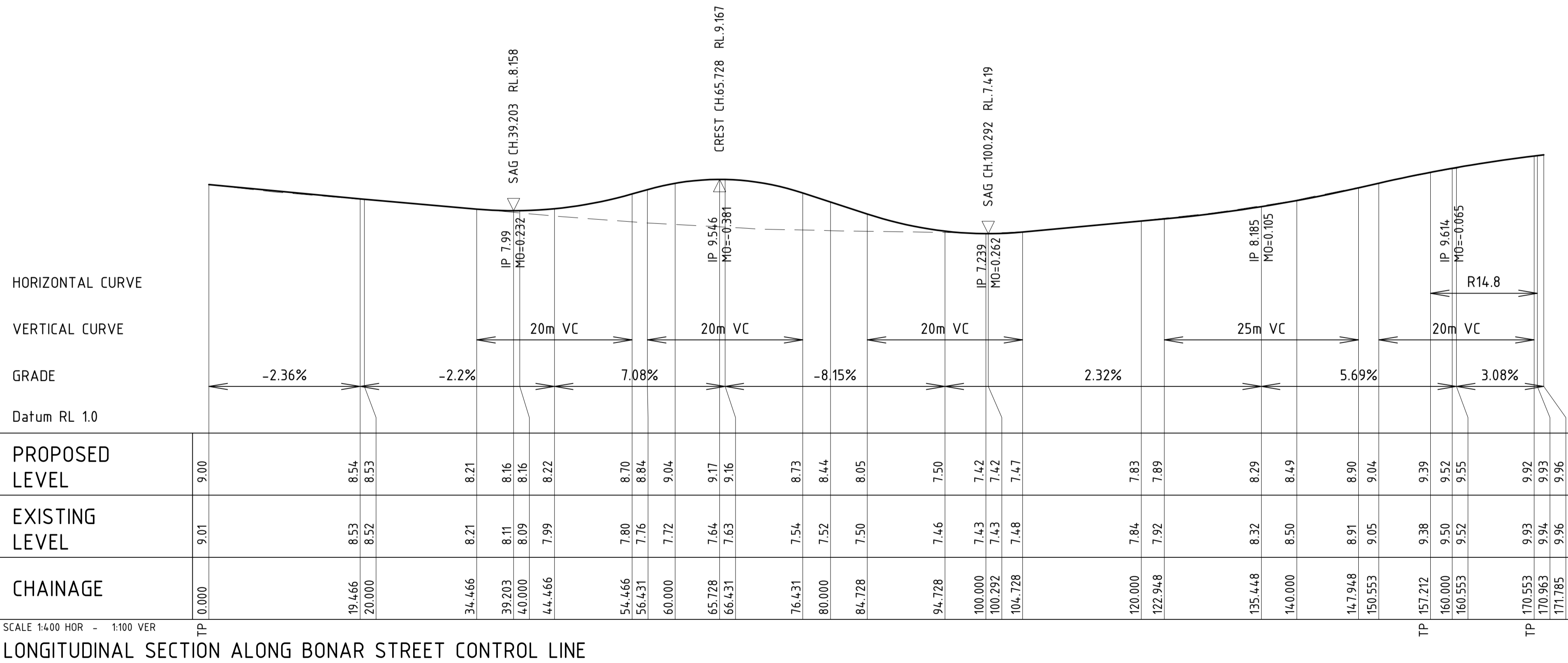
LONGITUDINAL SECTION ALONG BONAR STREET CONTROL LINE
