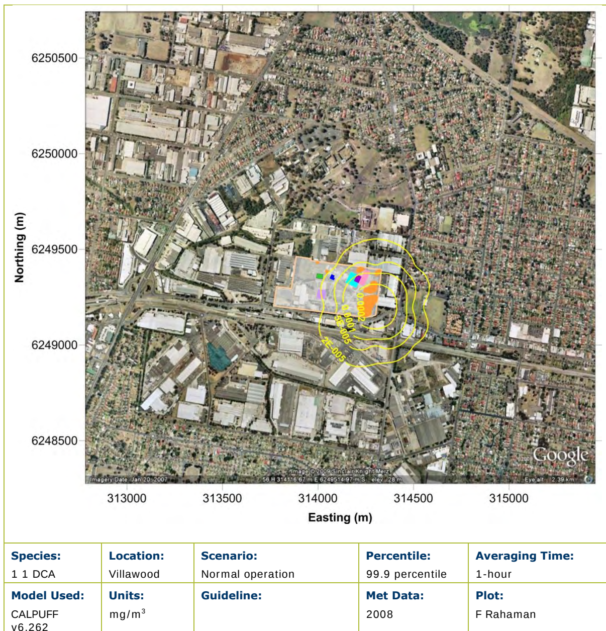
Figure C.10: Predicted 99.9 percentile 1-hour average 1,1-DCA increment due to the proposed operation
