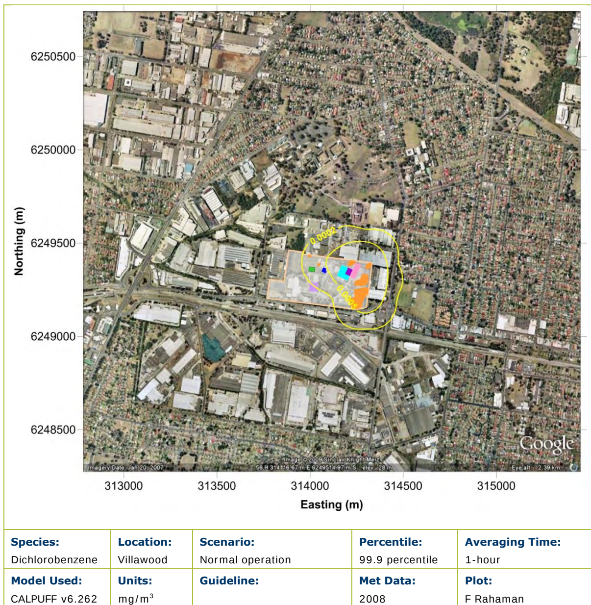
Figure C.5: Predicted 99.9 percentile 1-hour average dichlorobenzene increment due to the proposed operation
