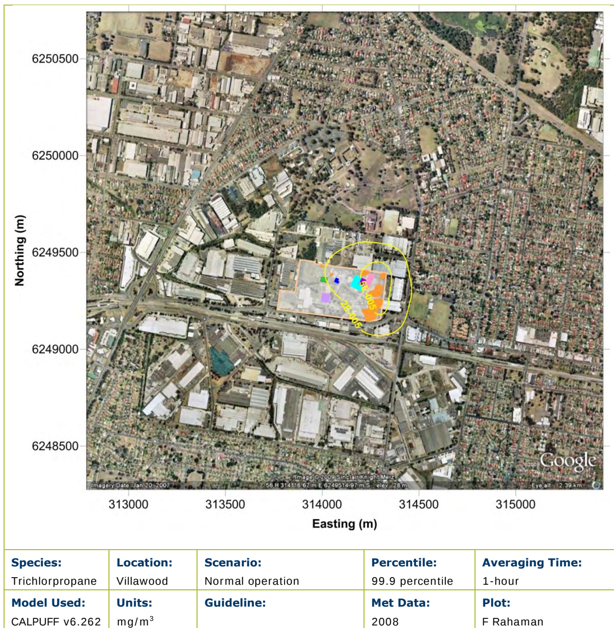
Figure C.8: Predicted 99.9 percentile 1-hour average trichloropropane increment due to the proposed operation
