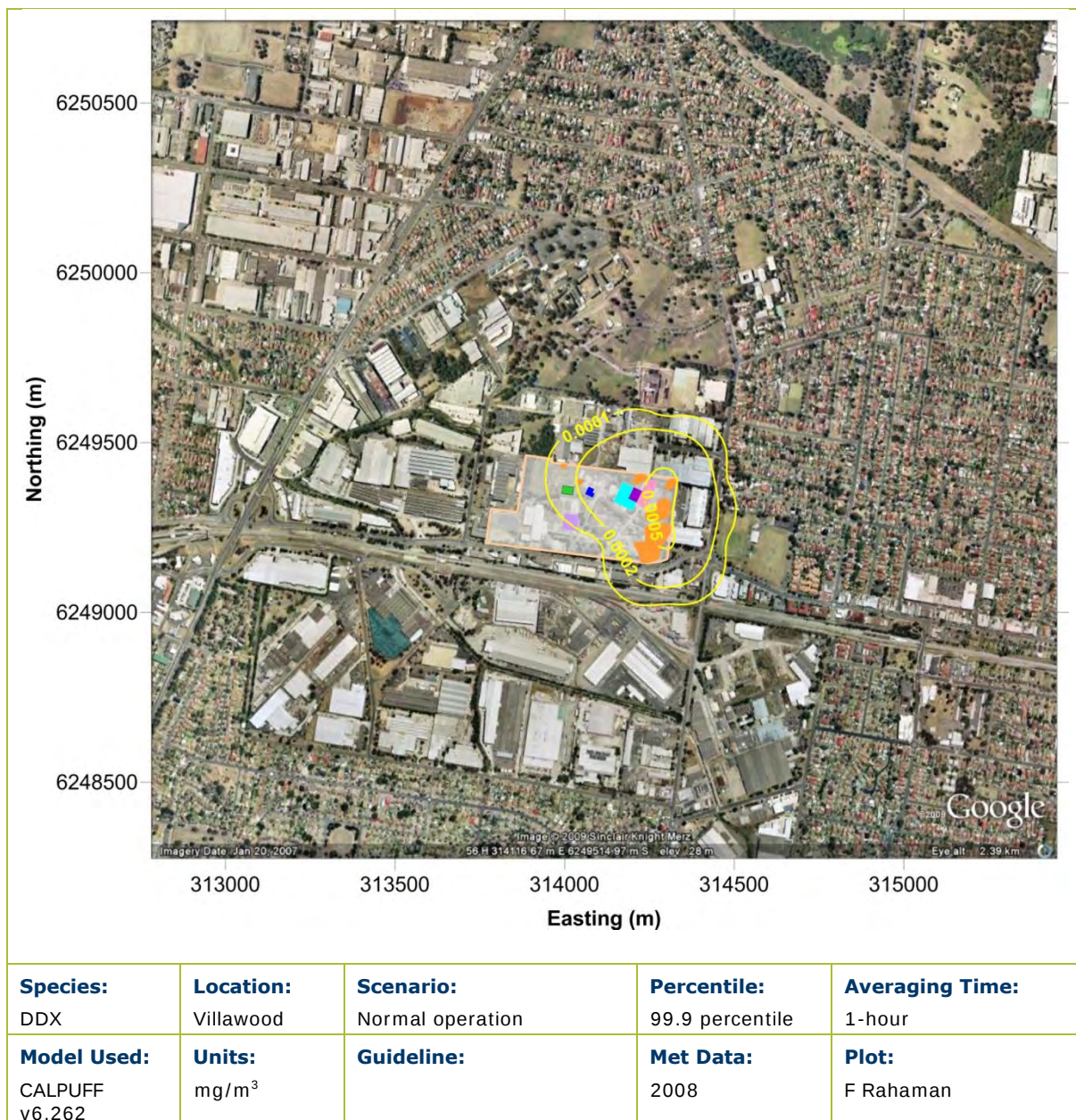
Figure C.1: Predicted 99.9 percentile 1-hour average DDX increment due to the proposed operation
