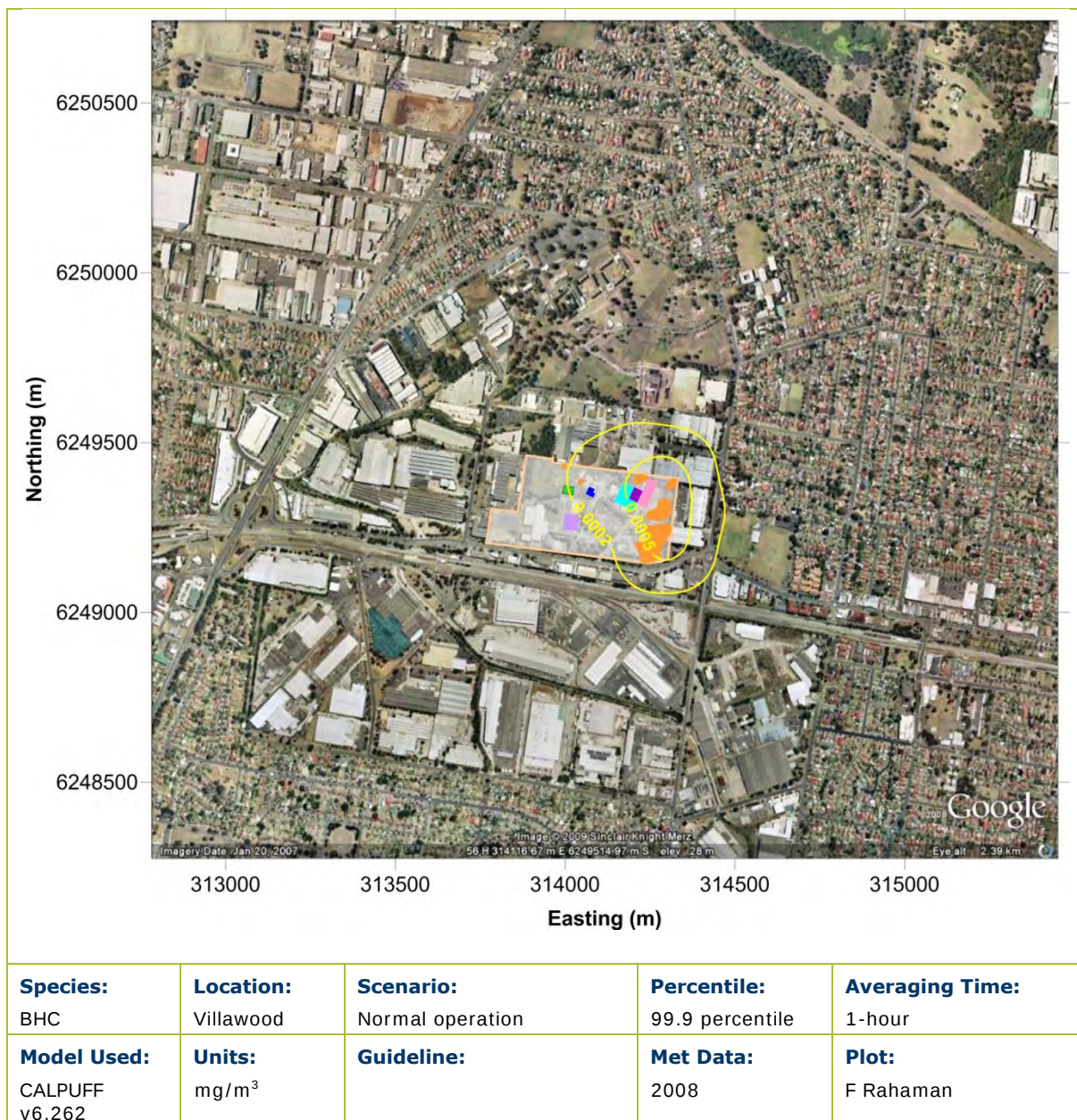
Figure C.9: Predicted 99.9 percentile 1-hour average BHC increment due to the proposed operation
