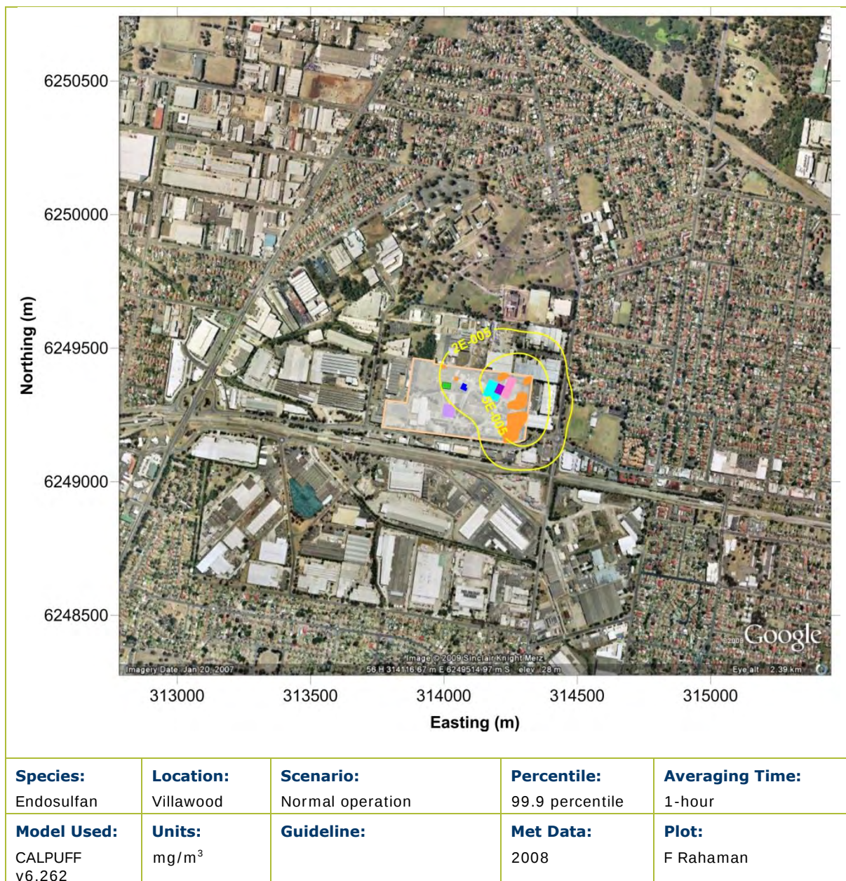
Figure C.4: Predicted 99.9 percentile 1-hour average endosulfan increment due to the proposed operation
