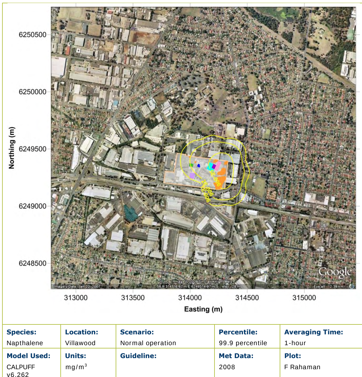
Figure C.2: Predicted 99.9 percentile 1-hour average naphthalene increment due to the proposed operation
