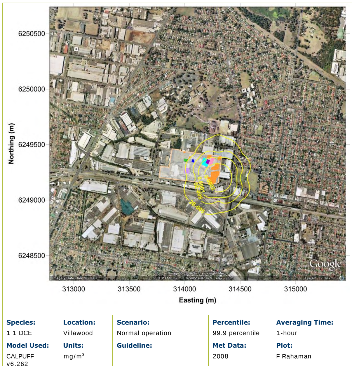
Figure C.11: Predicted 99.9 percentile 1-hour average 1,1-DCE increment due to the proposed operation
