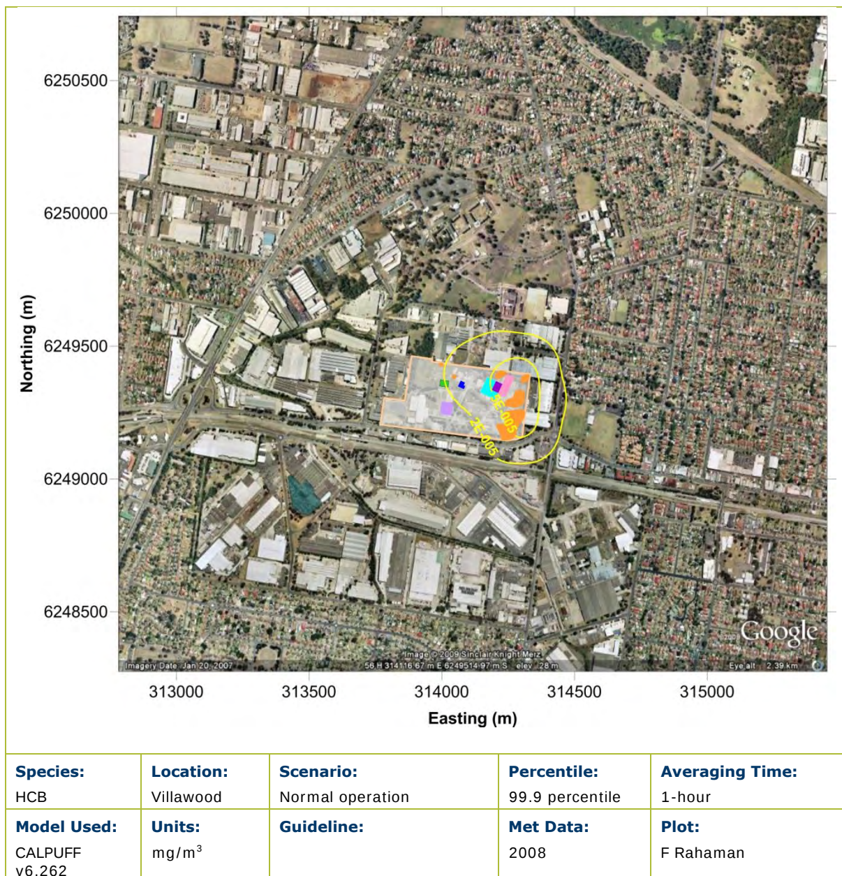
Figure C.7: Predicted 99.9 percentile 1-hour average HCB increment due to the proposed operation
