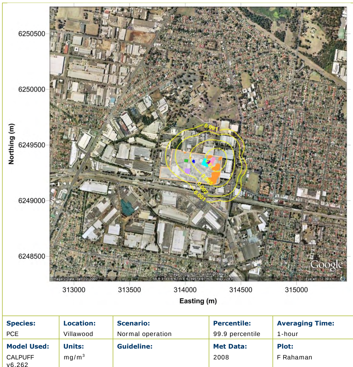
Figure C.3: Predicted 99.9 percentile 1-hour average PCE increment due to the proposed operation
