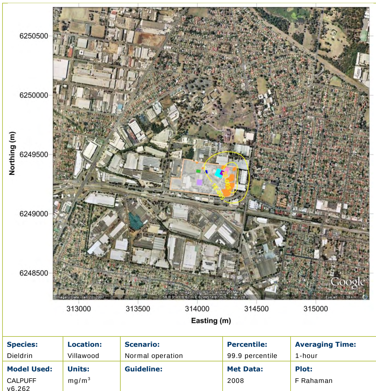
Figure C.6: Predicted 99.9 percentile 1-hour average dieldrin increment due to the proposed operation
