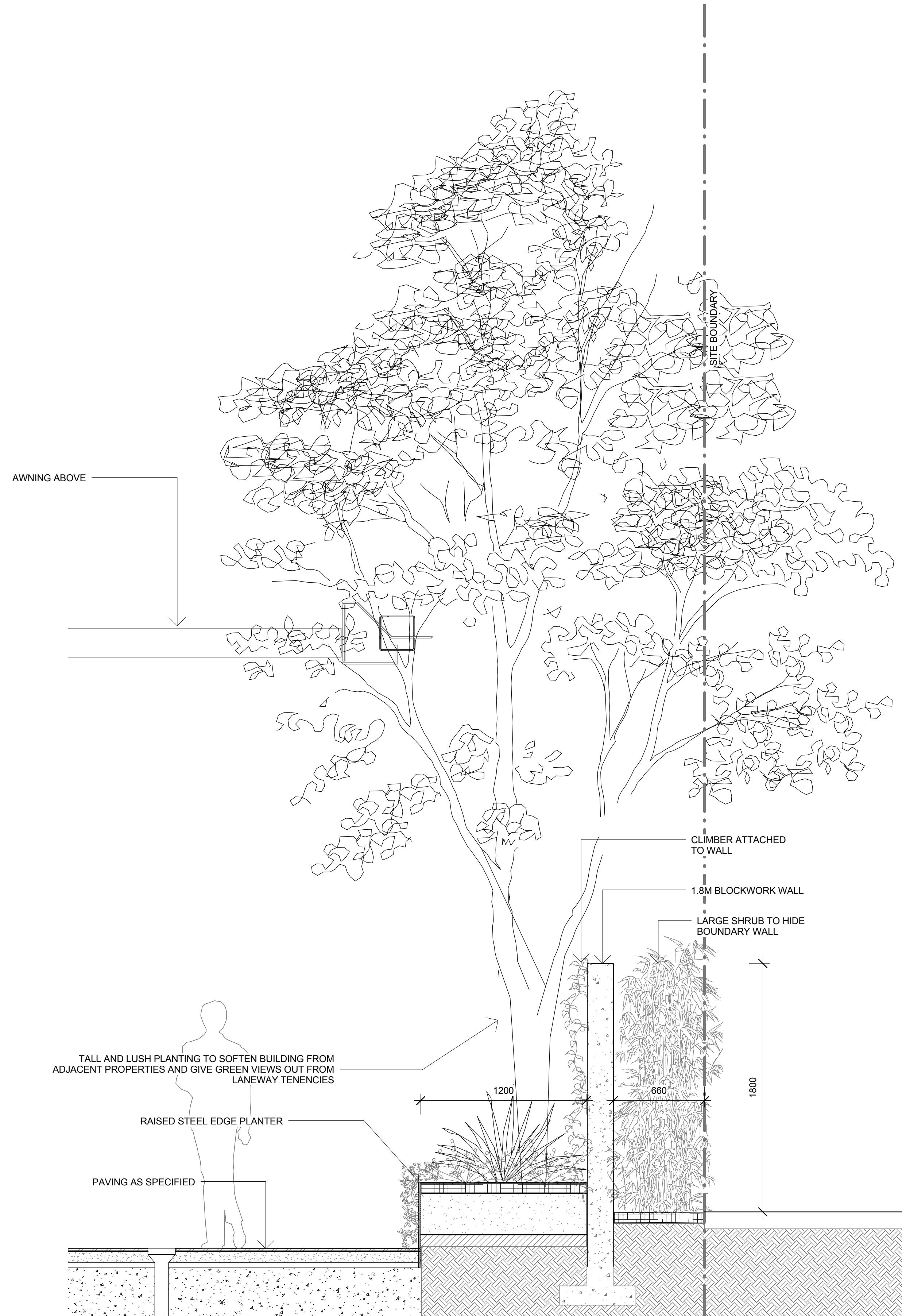
3 EASTERN LANEWAY BOUNDARY WALL 1 : 20
