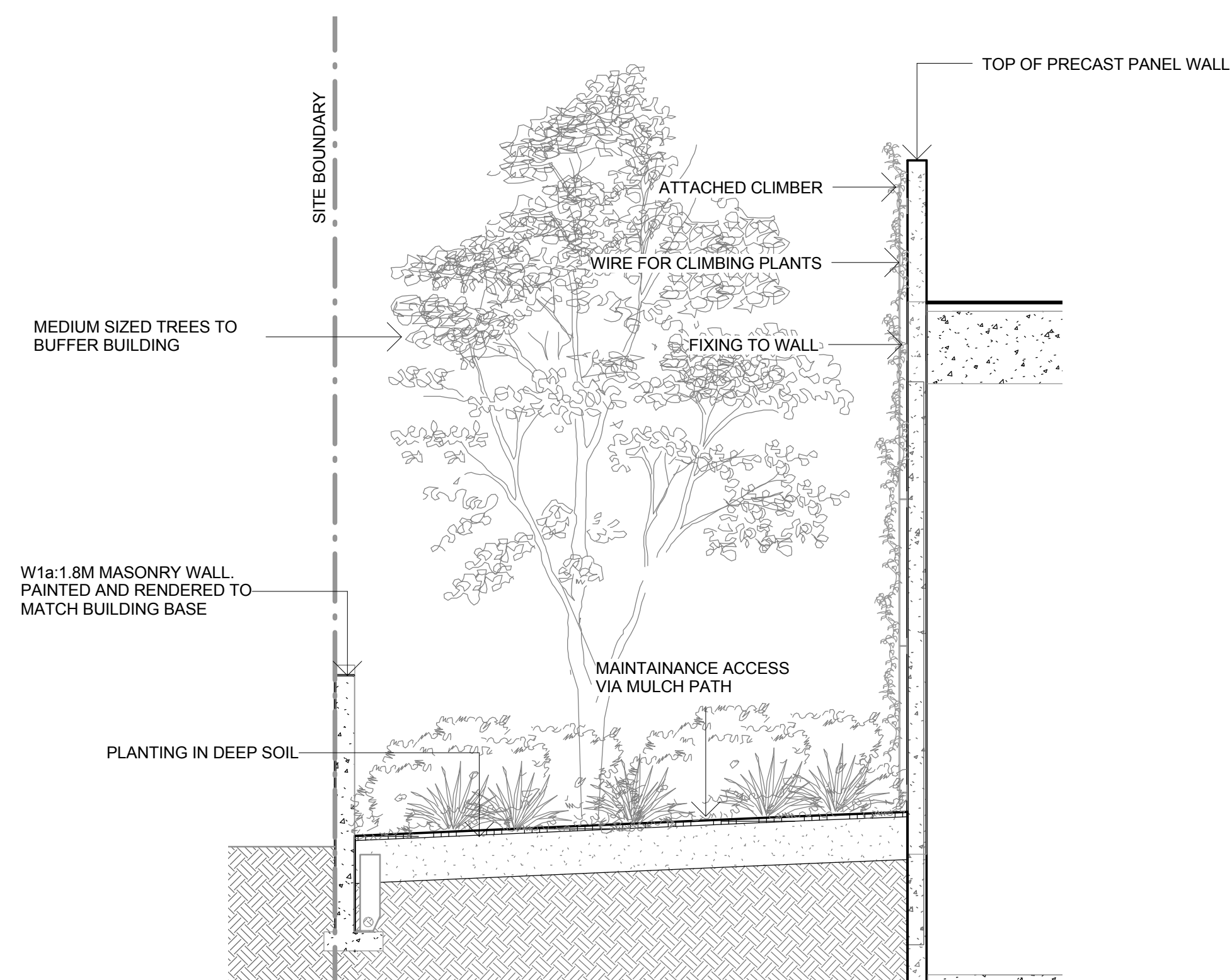
1 WESTERN BOUNDARY WALL 1 : 50
