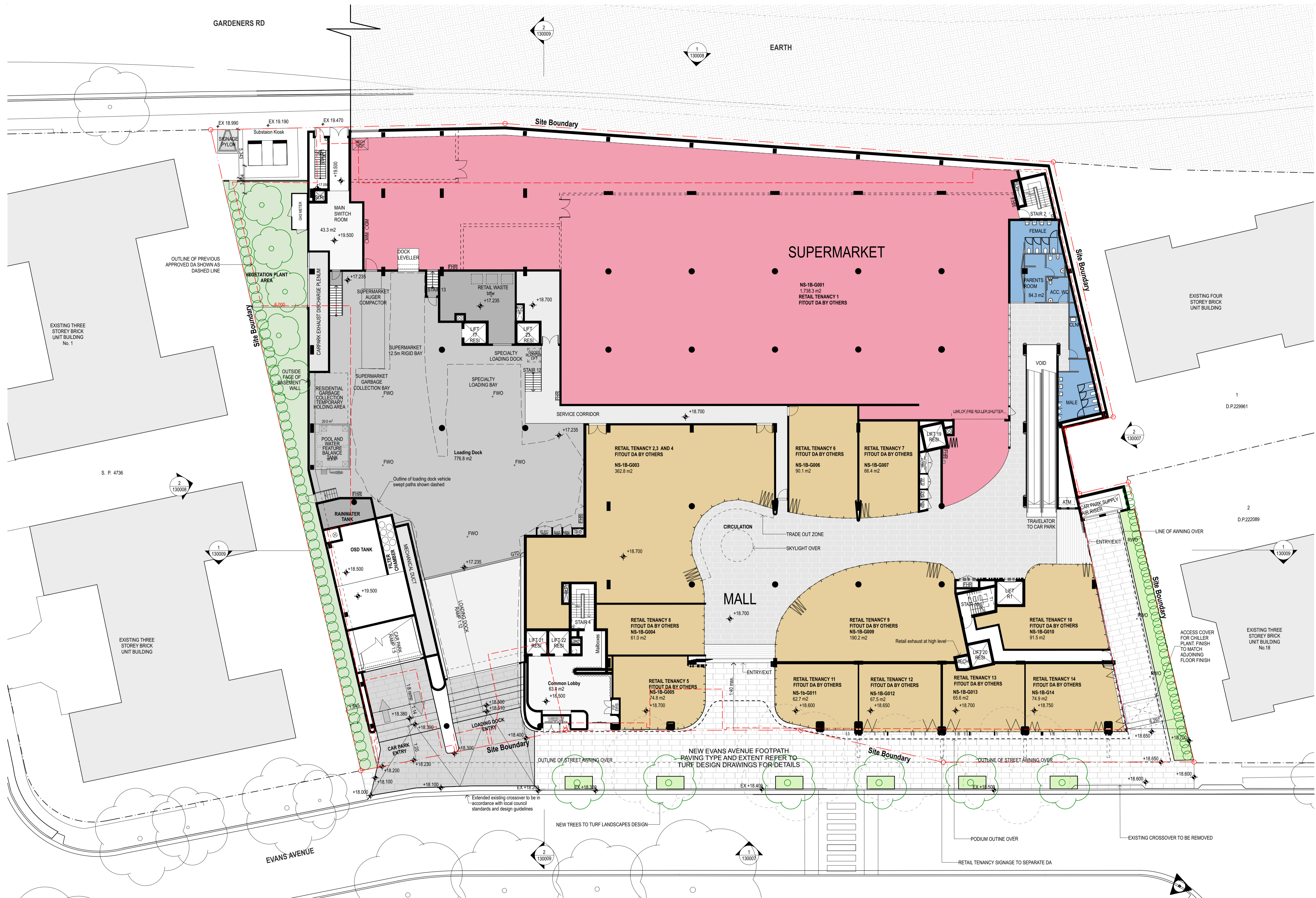
1 PLAN Ground Floor 1:200
