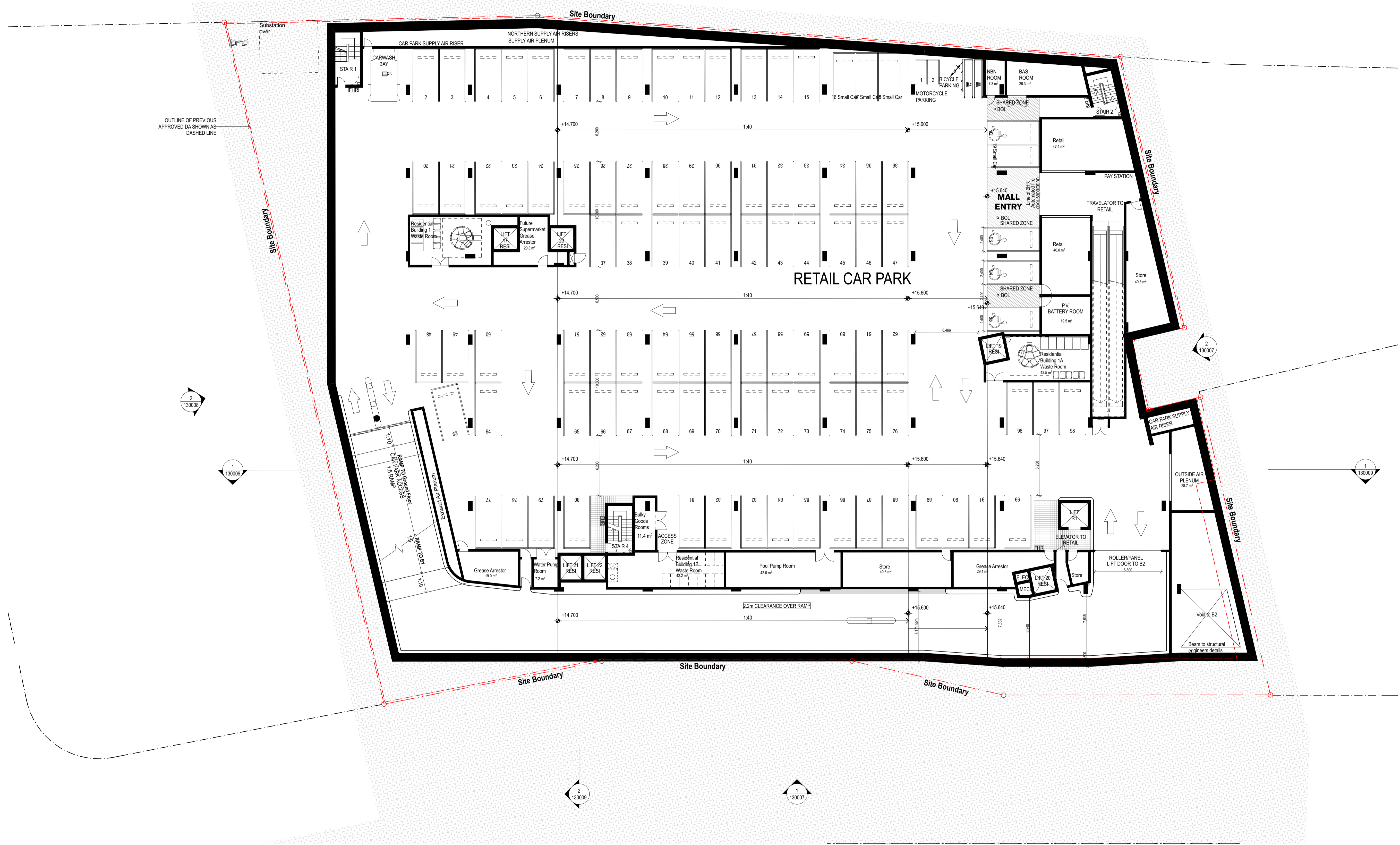
1 PLAN Basement Level 1 1:200
