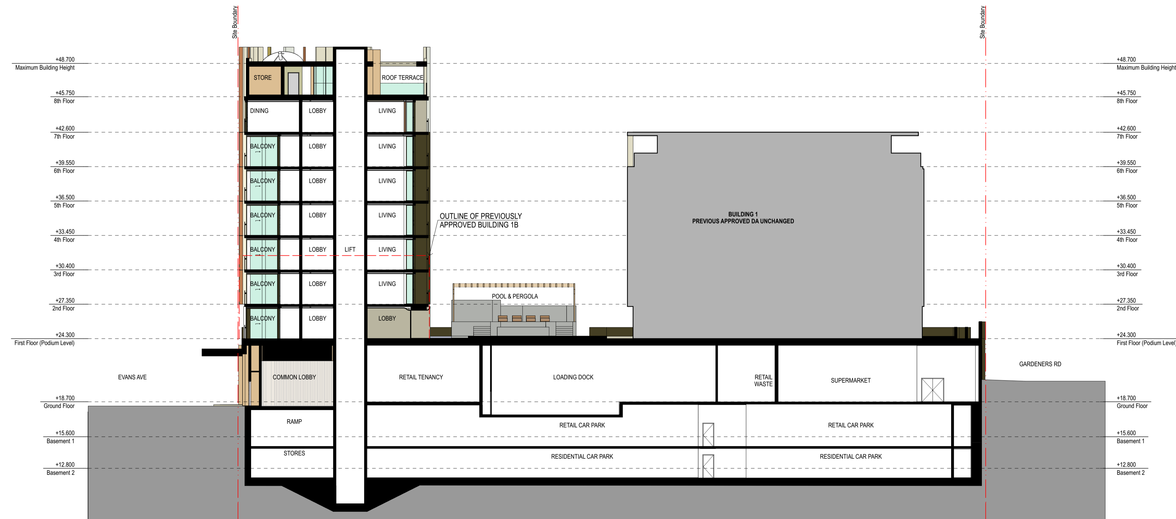
2 SECTION 2 1:200
