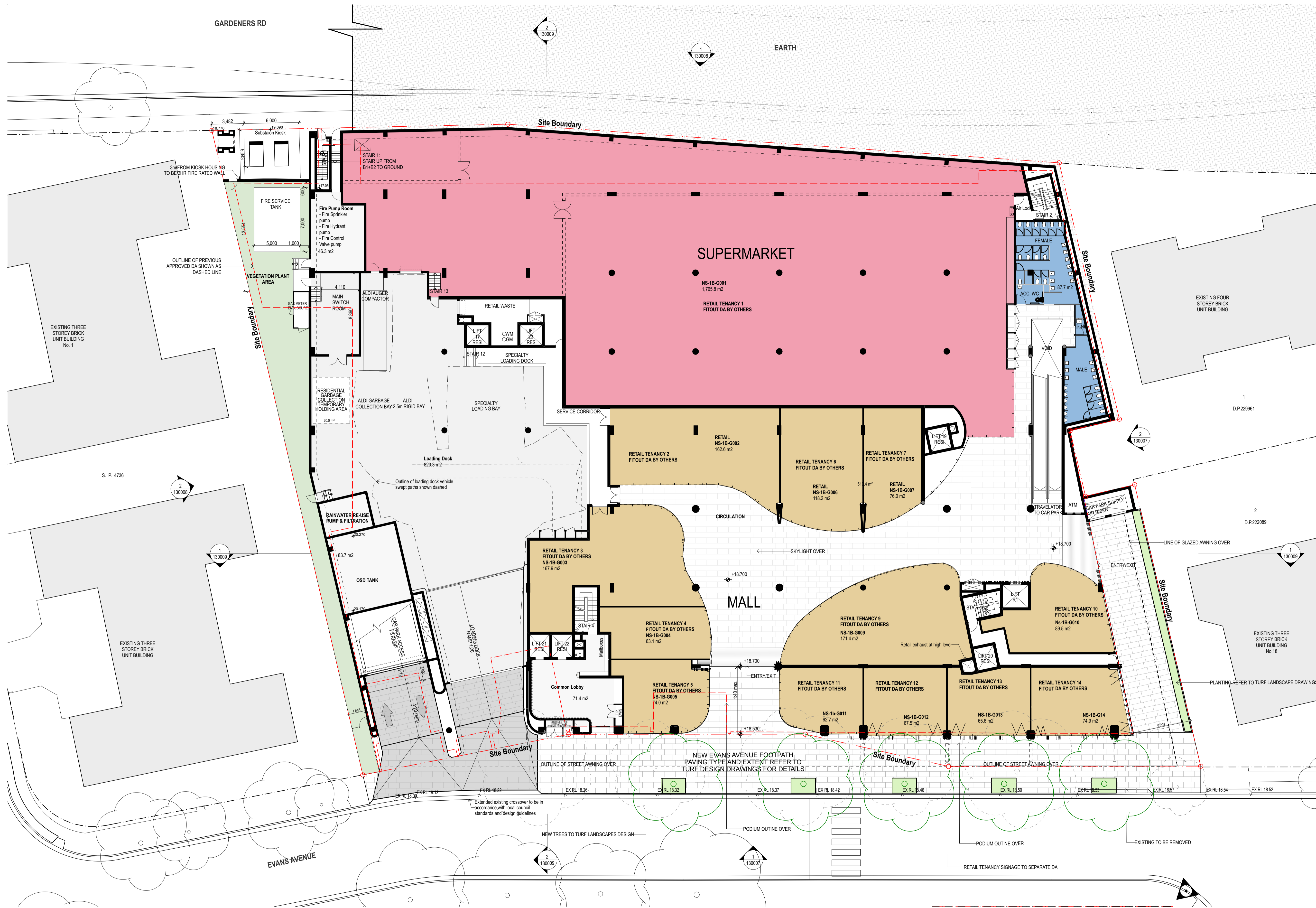
1 PLAN Ground Floor 1:200
