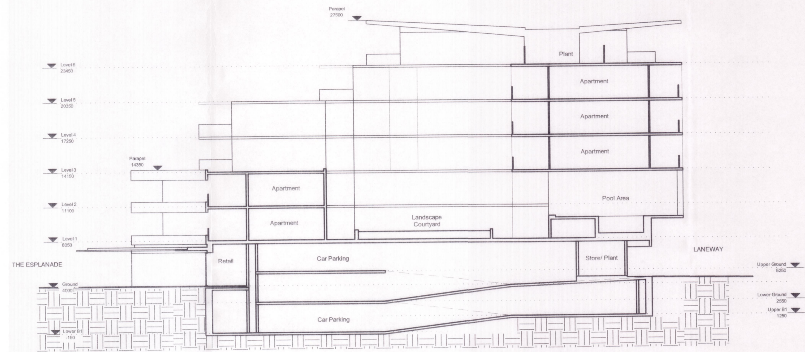
SECTION 01 1:2000A1
