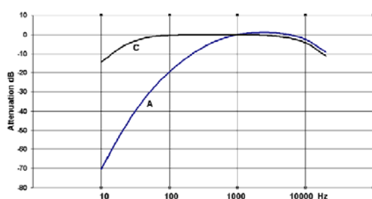
Figure 1: Sound Level Meter Weighting Curves A and C; Figure 2: G-Weighting for Infrasound
