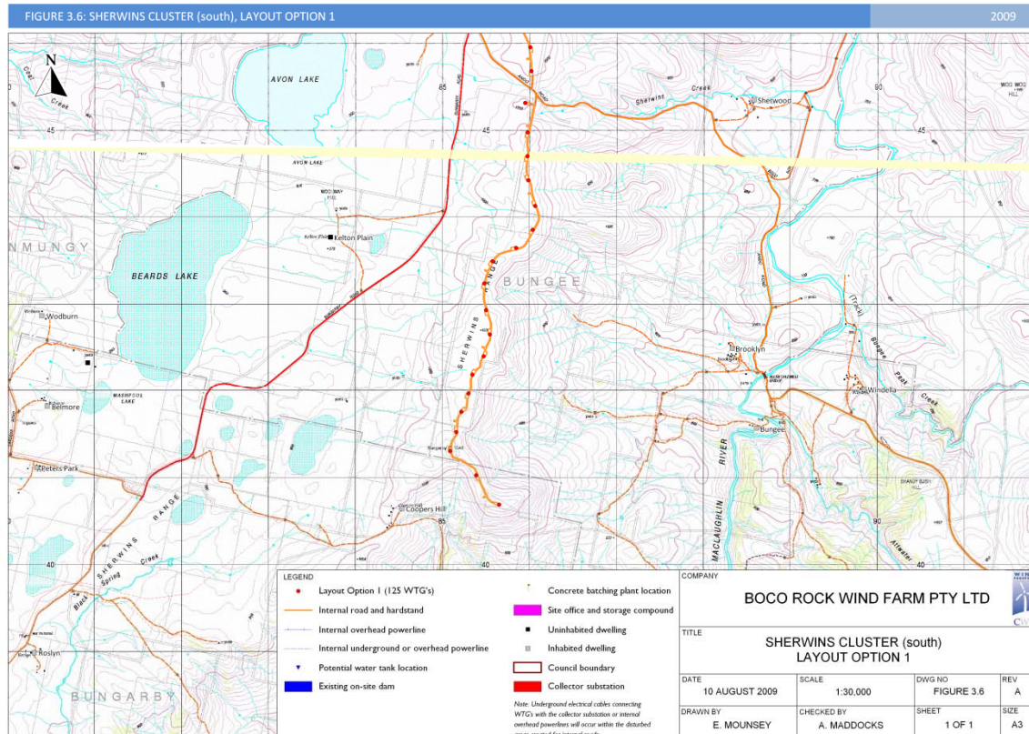
Figure 3.6 Sherwins Cluster (south), Layout Option 1 (A3 size versions of these Figures are displayed in Volume 2)
