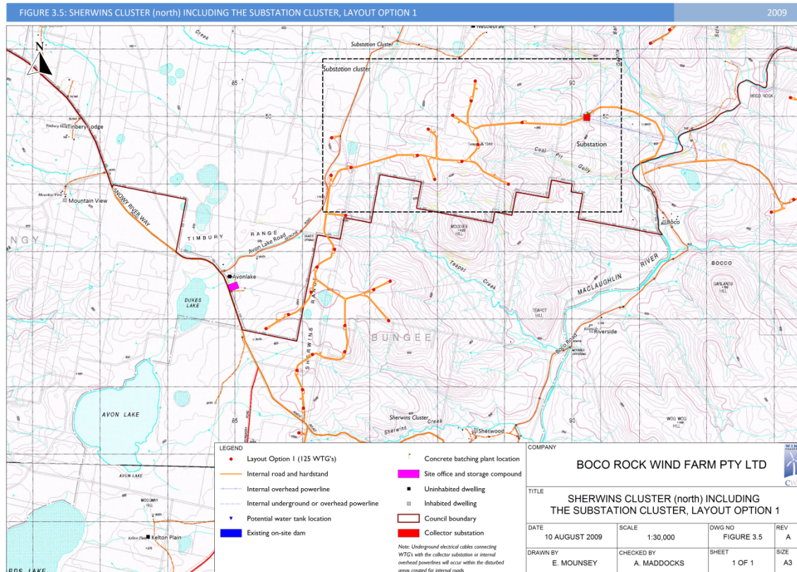
Figure 3.5 Sherwins Cluster (north), including the 'substation Cluster', Layout Option 1
