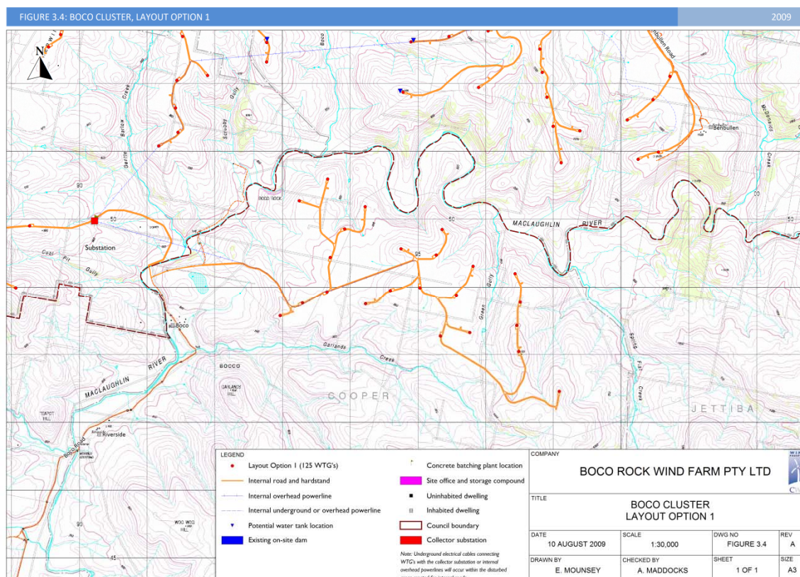
Figure 3.4 Boco Cluster, Layout Option 1
