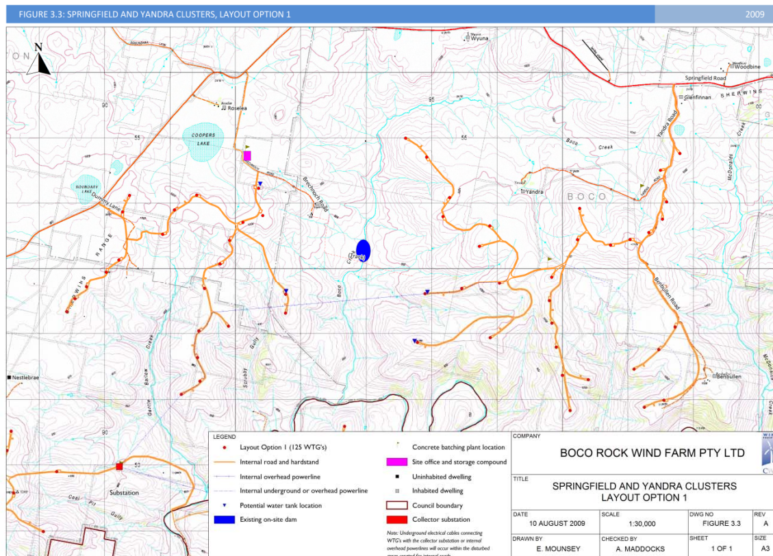
Figure 3.3 Springfield and Yandra Clusters, Layout Option 1
