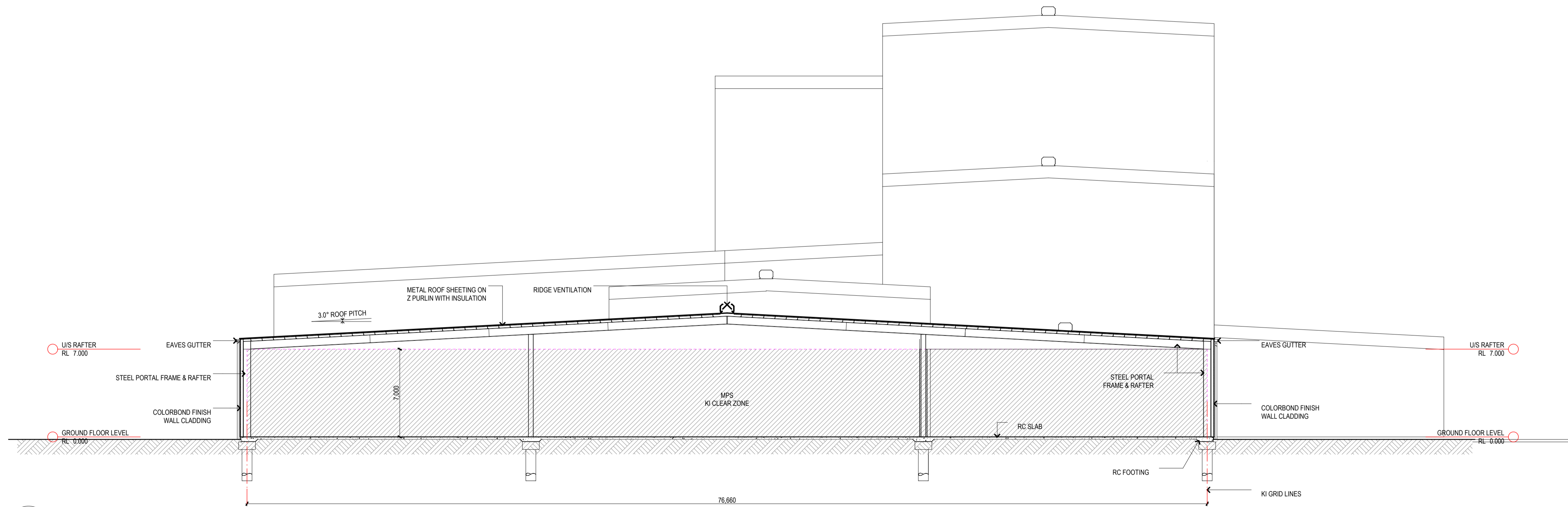
2 SECTION SCALE 1:200
