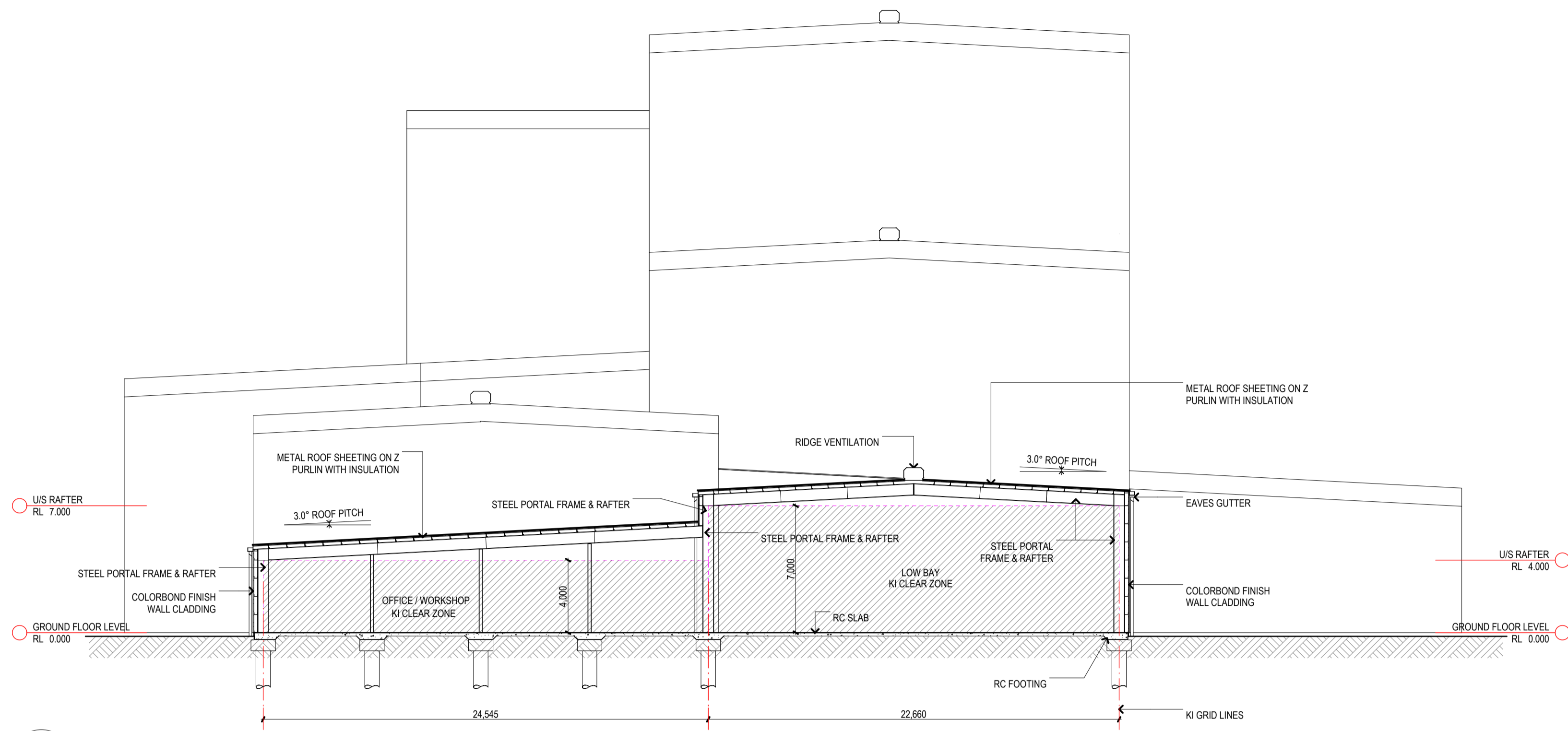
1 S-01 SECTION SCALE 1:200
