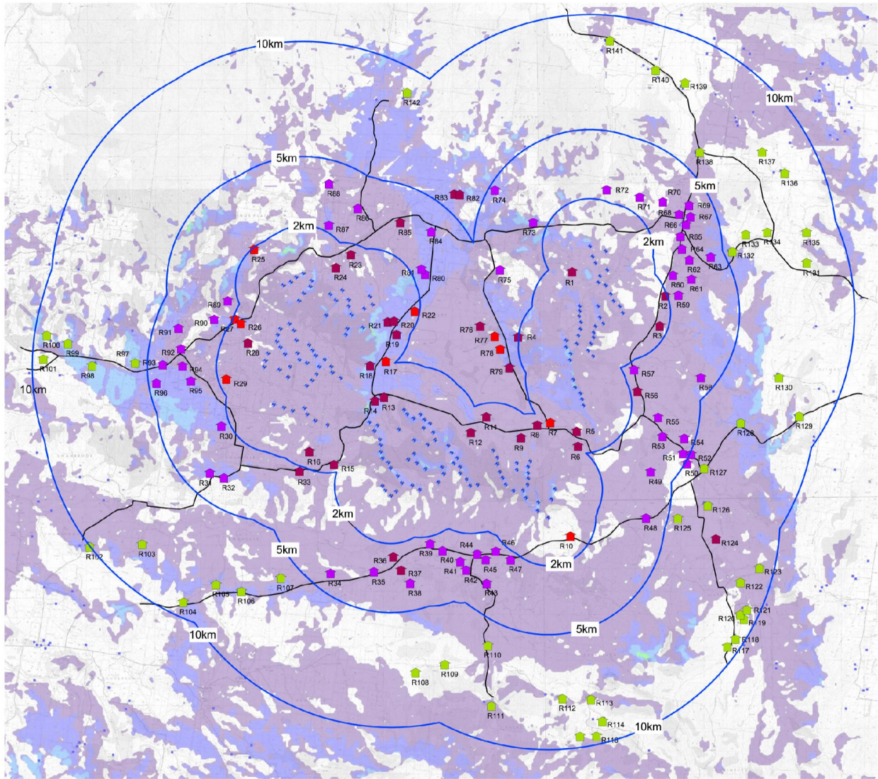
SAPPHIRE WIND FARM - '80m' DESIGN LAYOUT, ZONE OF VISUAL INFLUENCE, WHOLE TURBINE
