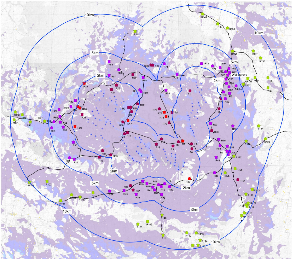
SAPPHIRE WIND FARM - '110m' DESIGN LAYOUT, ZONE OF VISUAL INFLUENCE, WHOLE TURBINE
