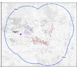
General location plan - PM11 (Turbine locations are indicative only)
