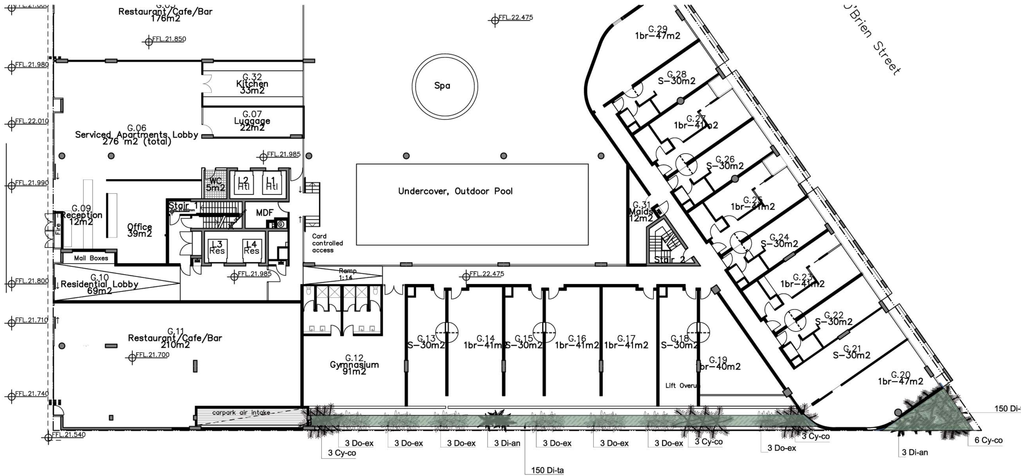
LEVEL 00 - SERVICED APARTMENTS REFER TO LA01 FOR HALL STREET AND O'BRIEN STREET STREETSCAPE REFER TO LA02 FOR GROUND FLOOR LANDSCAPE PLAN
