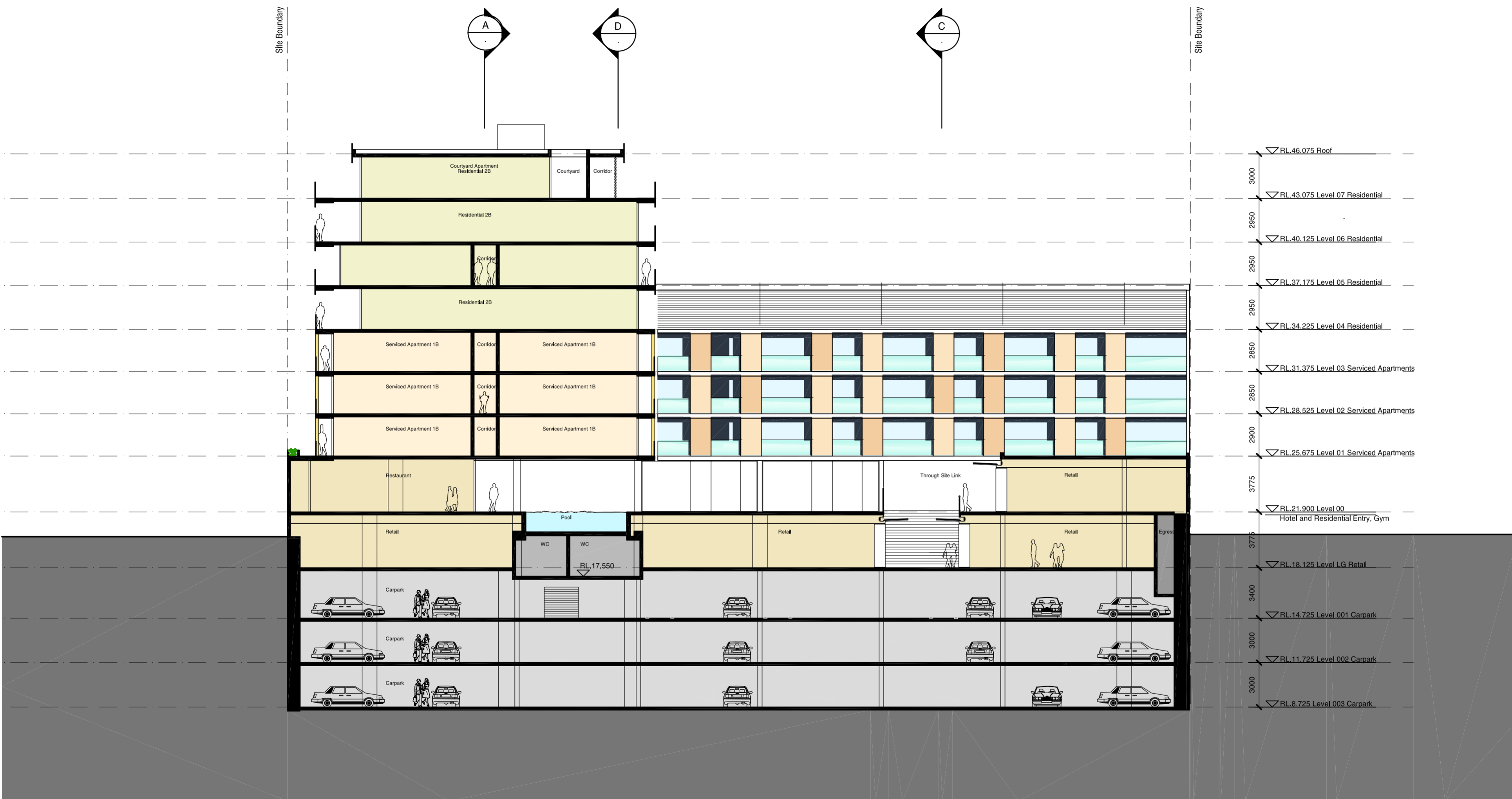
1 Section FF 1:200
