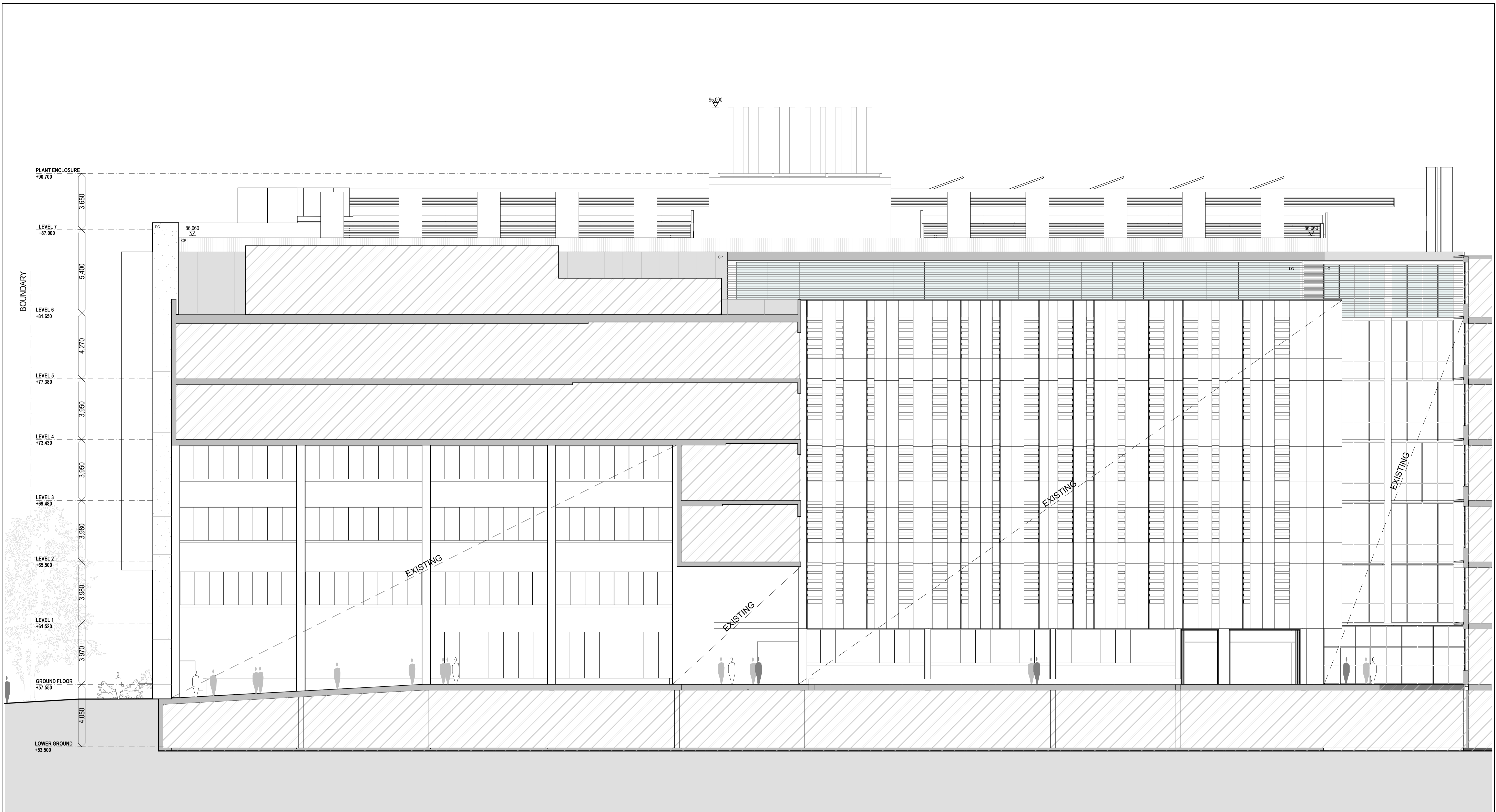
1 West Elevation 1:100
