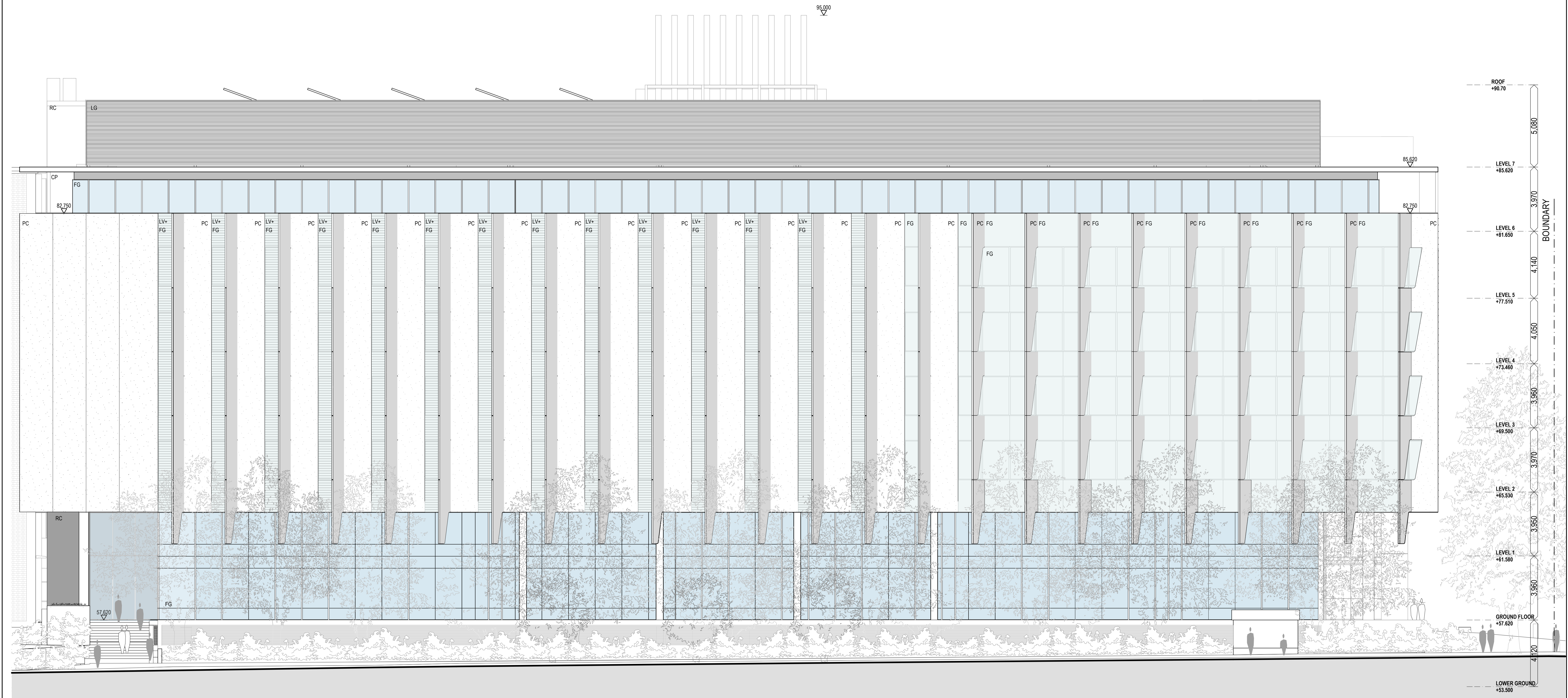
1 East Elevation - Botany Street 1:100
