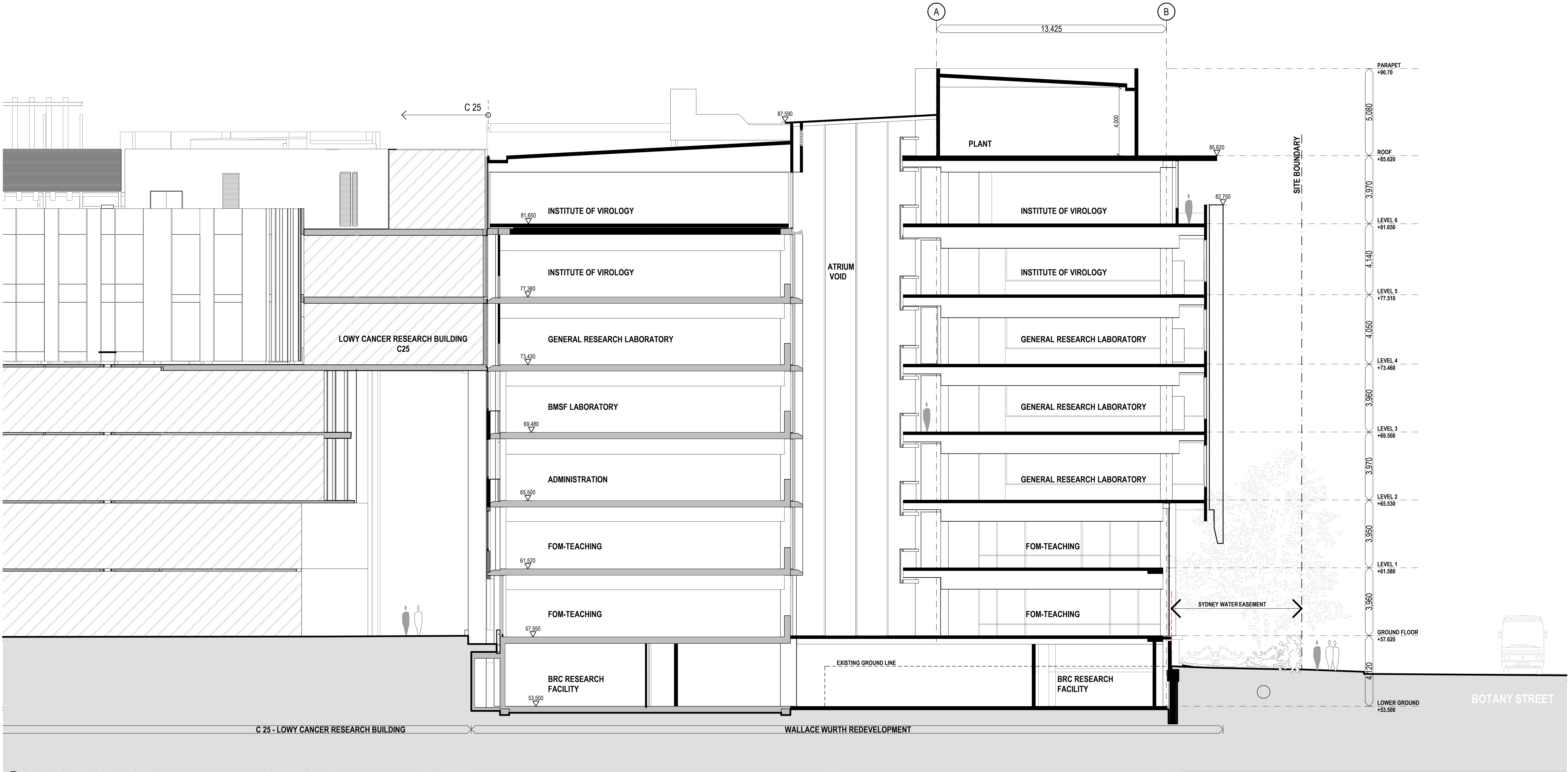
1 Cross Section A 1:100
