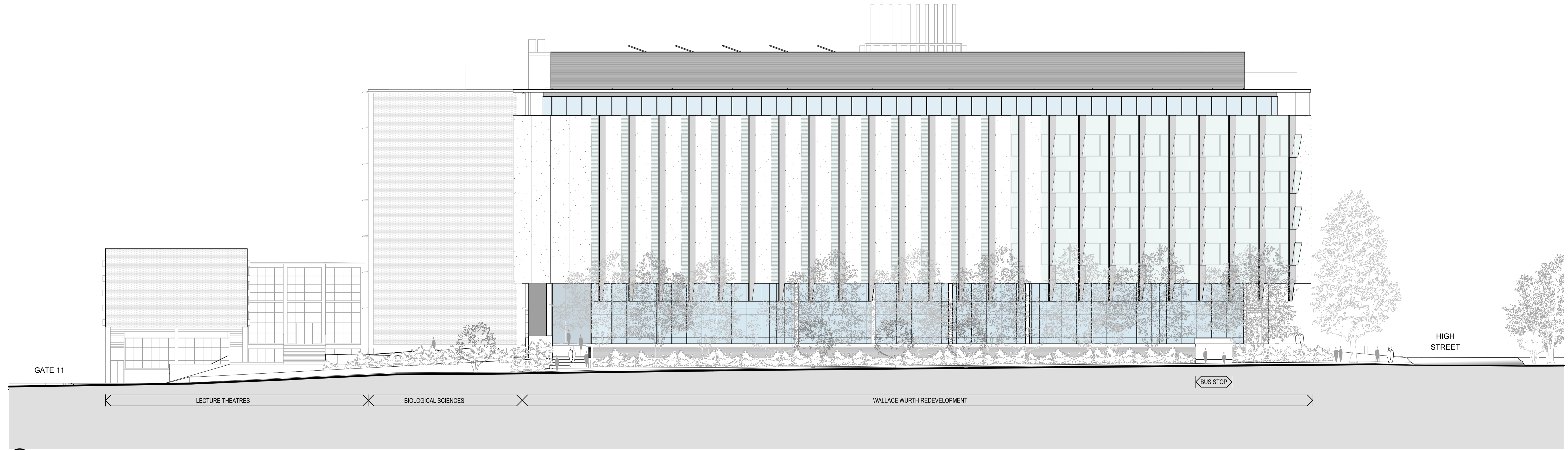
2 Street Scape - Botany Street 1:200
