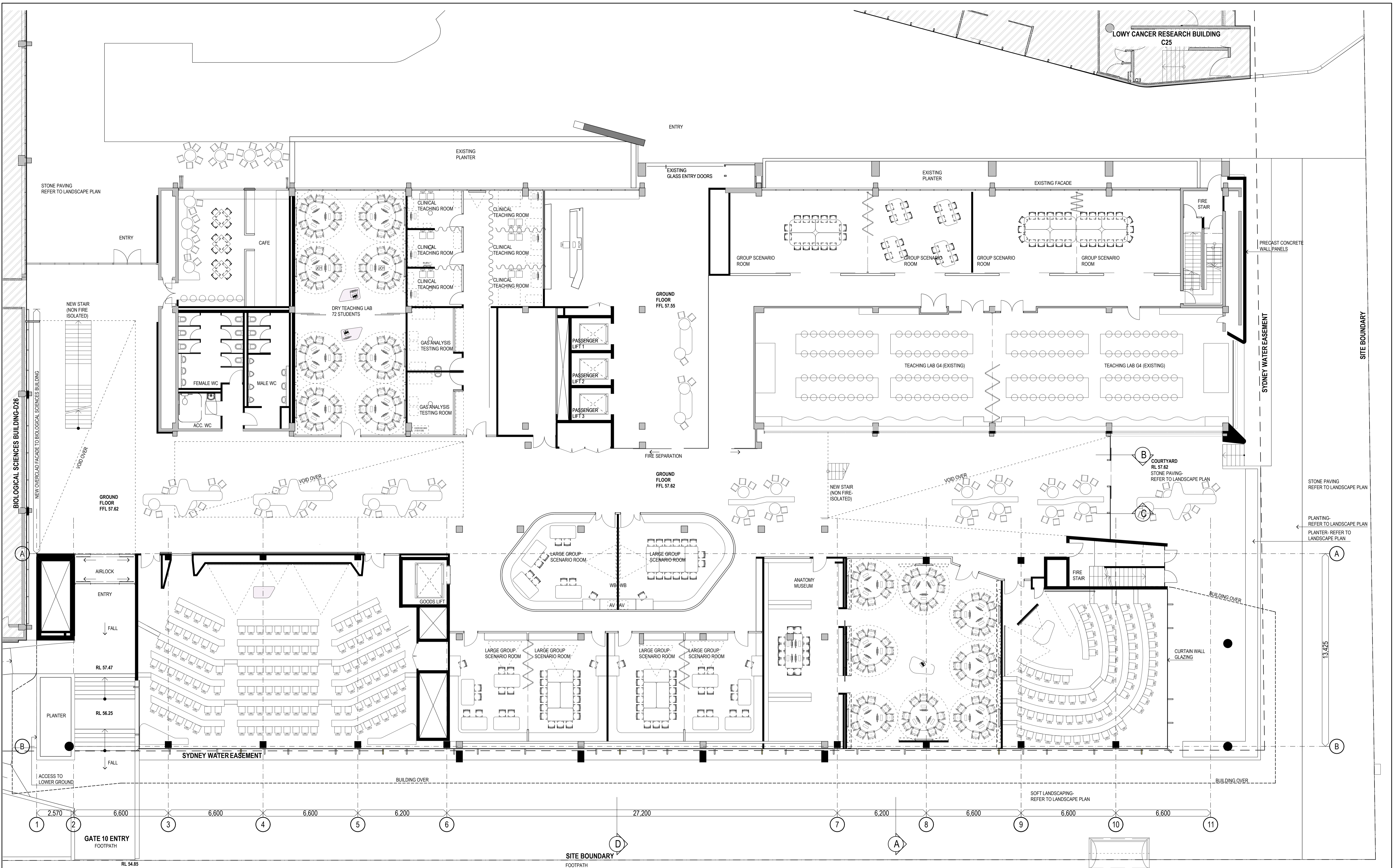
1 Ground Floor 1:100
