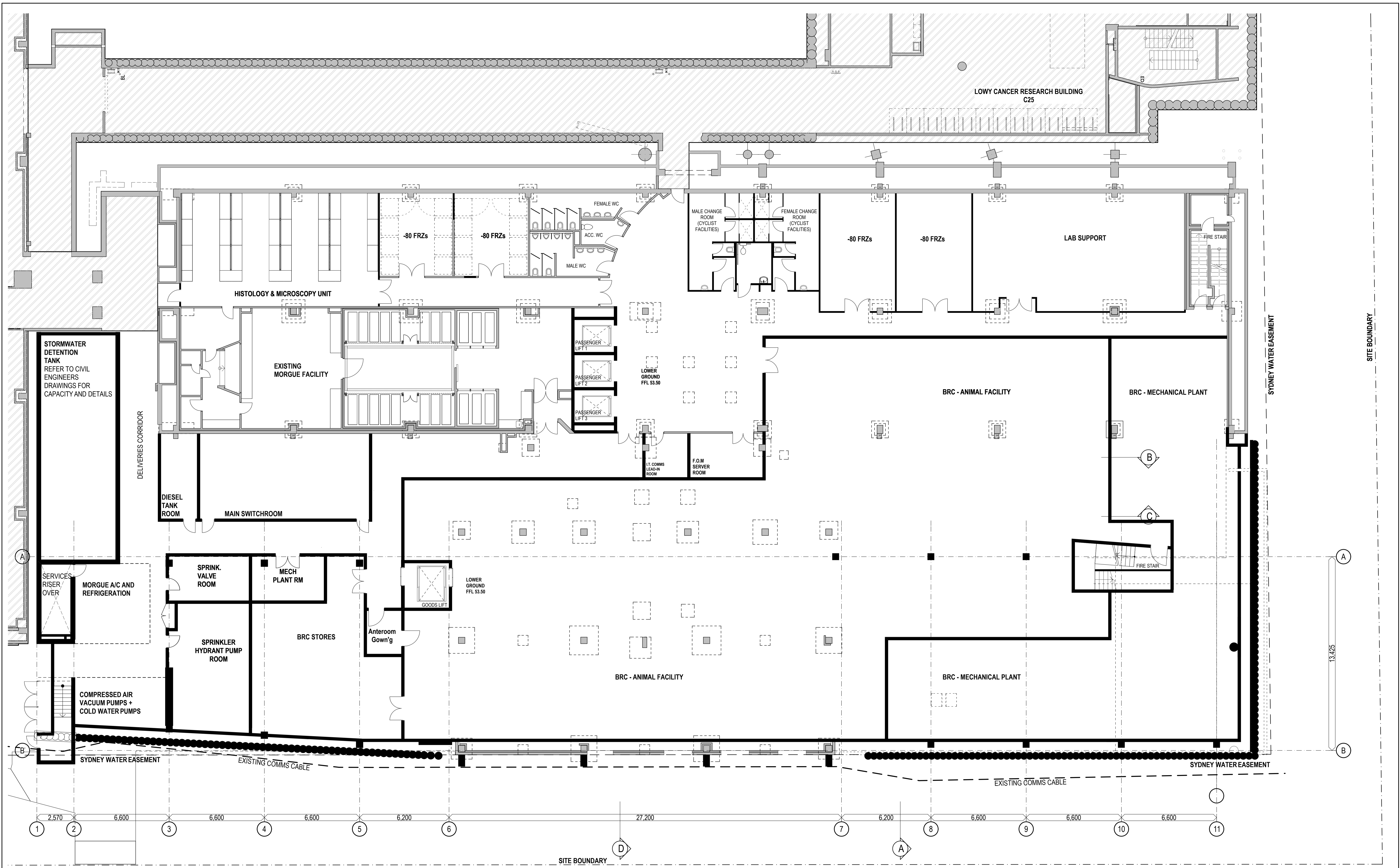
1 Lower Ground Floor (MW 53500) 1:100
