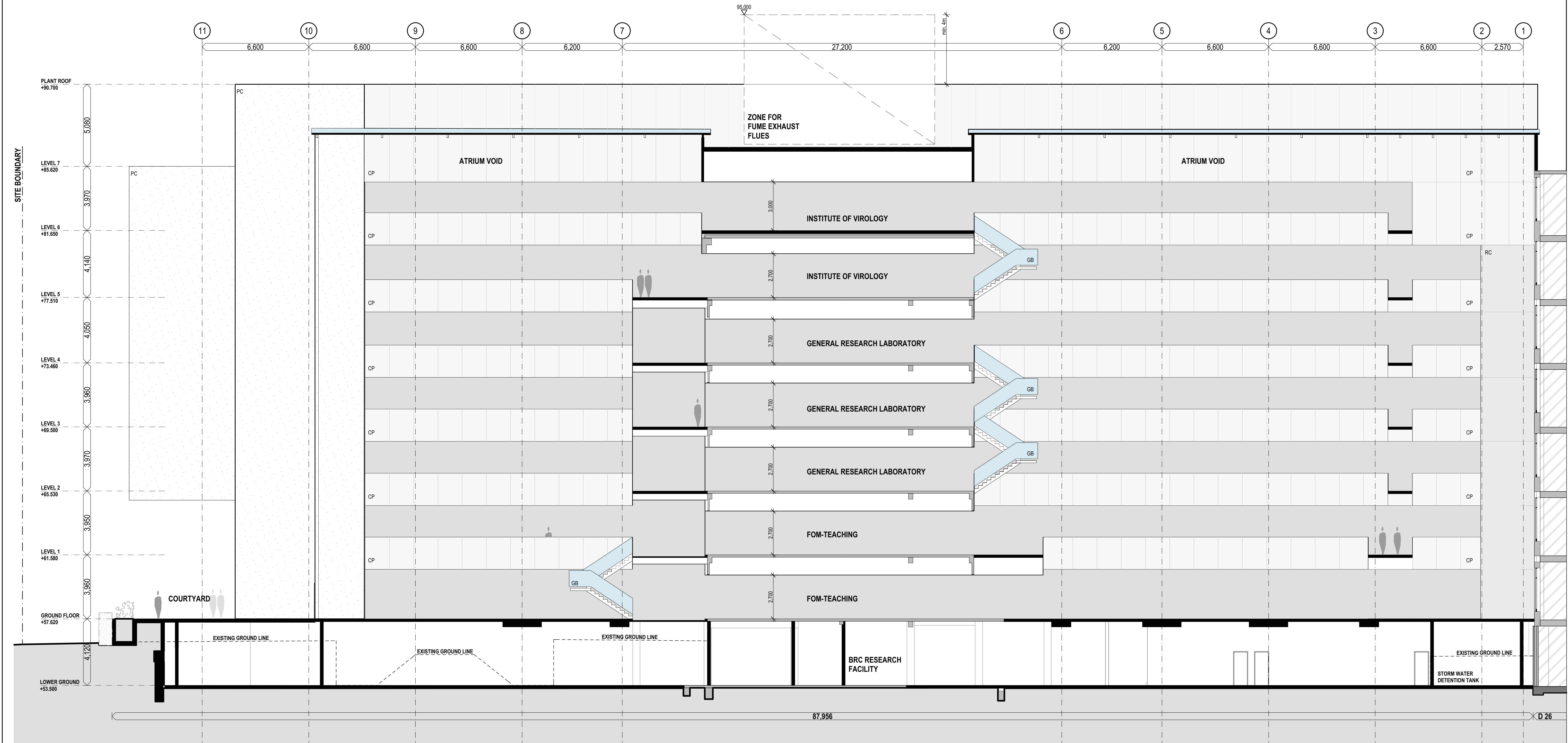
1 Long Section B (looking east) 1:100
